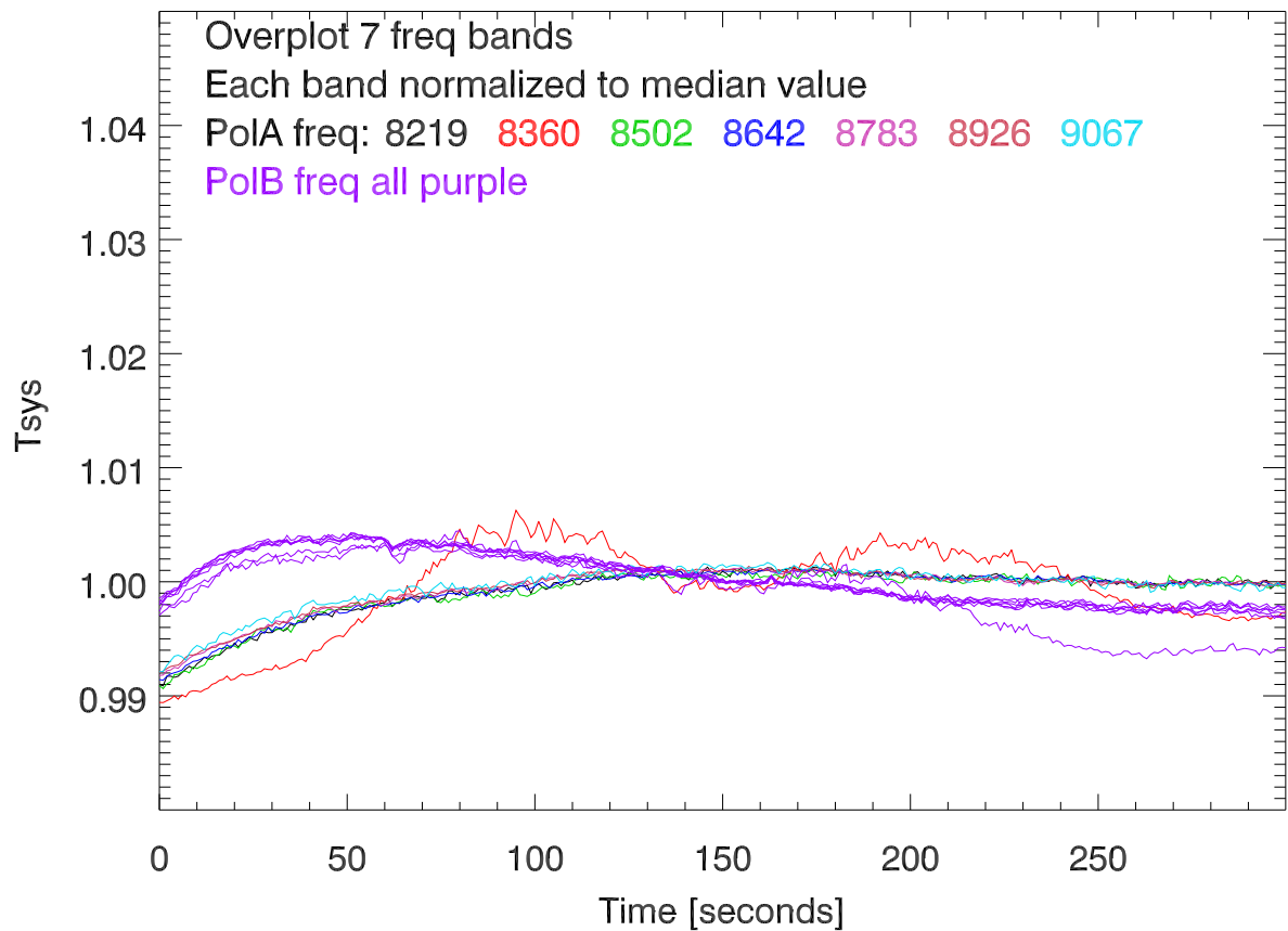
Relative Tsys change vs time for B0833-45
