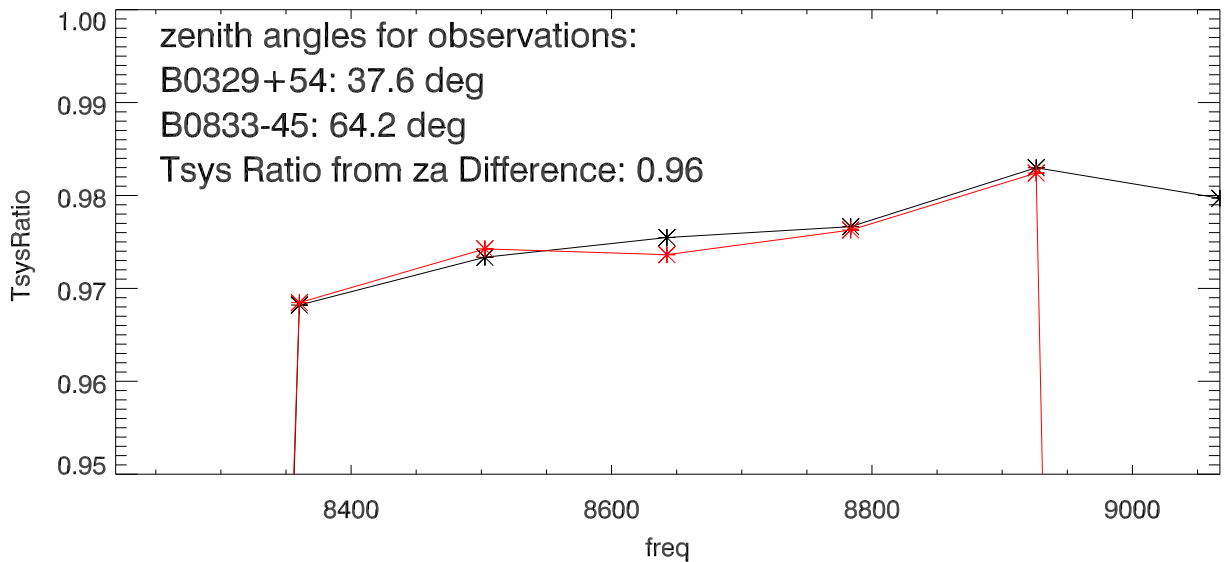
Median Tsys Ratio B0329+54/B0833-45 by frequency
