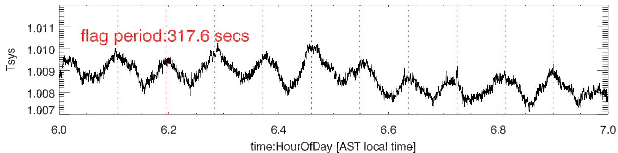
Blowup showing ripple
