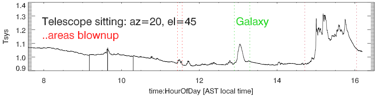
14mar16 12meter xband total power vs time
