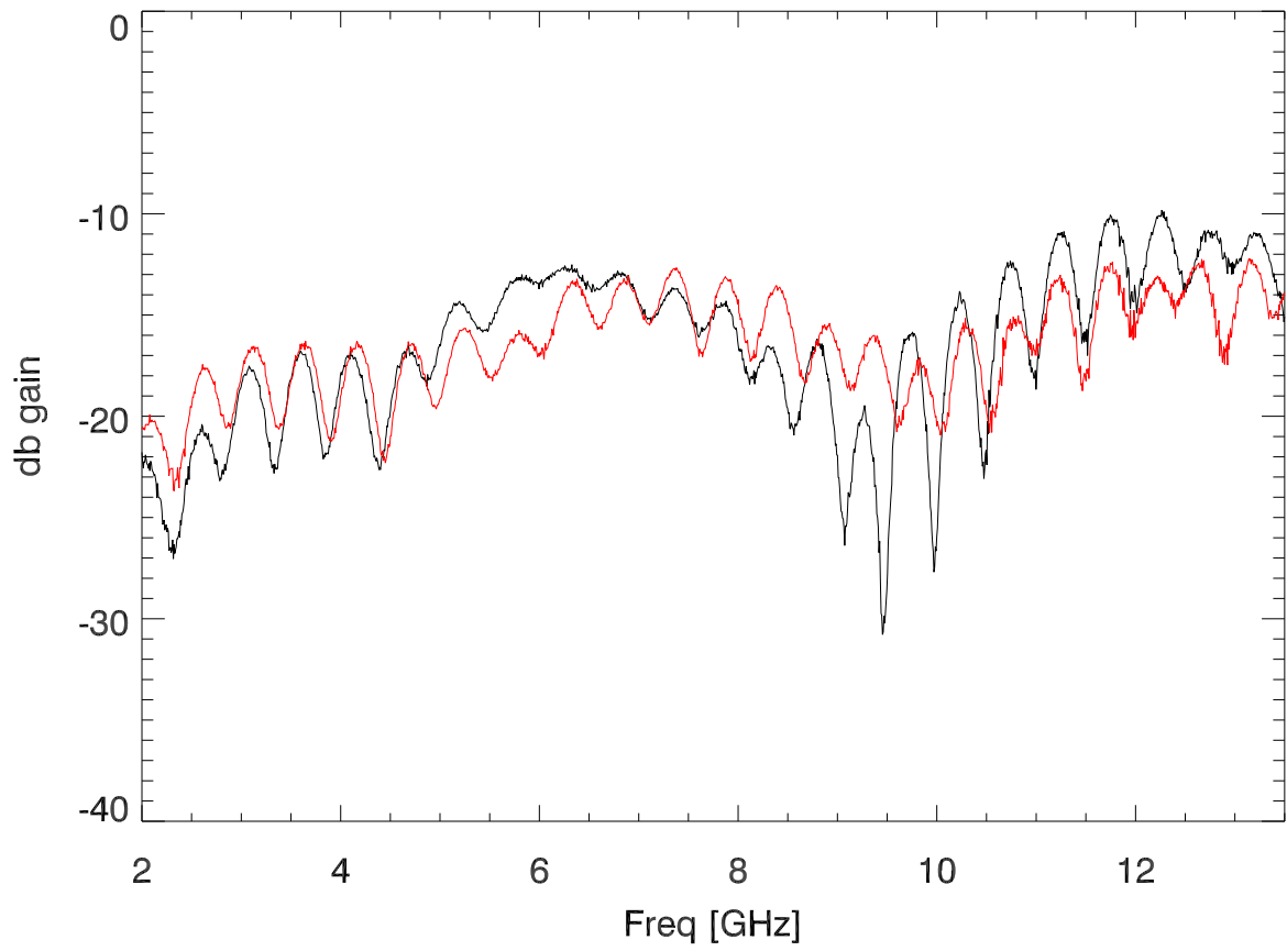
S11 vs freq. (reflected from PoIA input)
