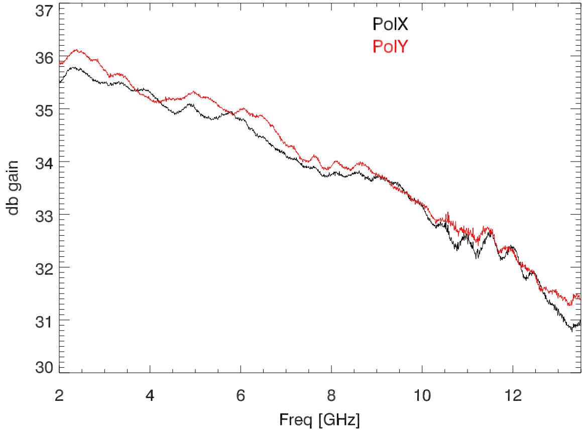
15may23 S21 vs freq RF_FIBER_THRU
