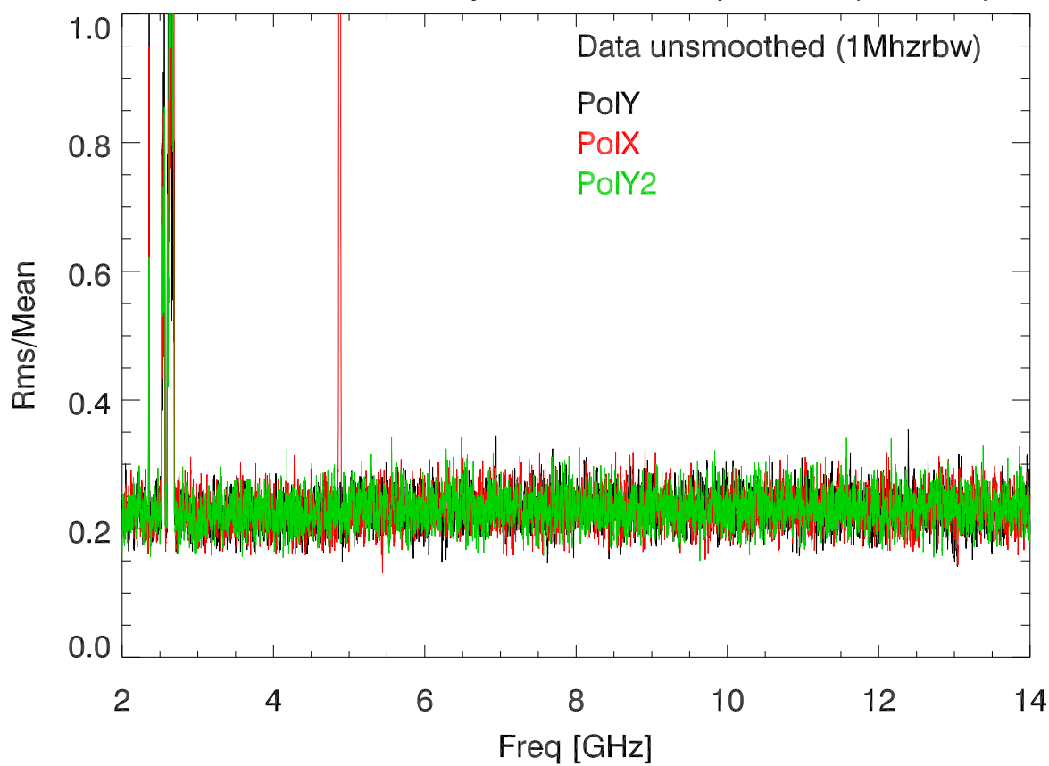
Rms/mean be freq chan for 10 spectra. (on Abs)
