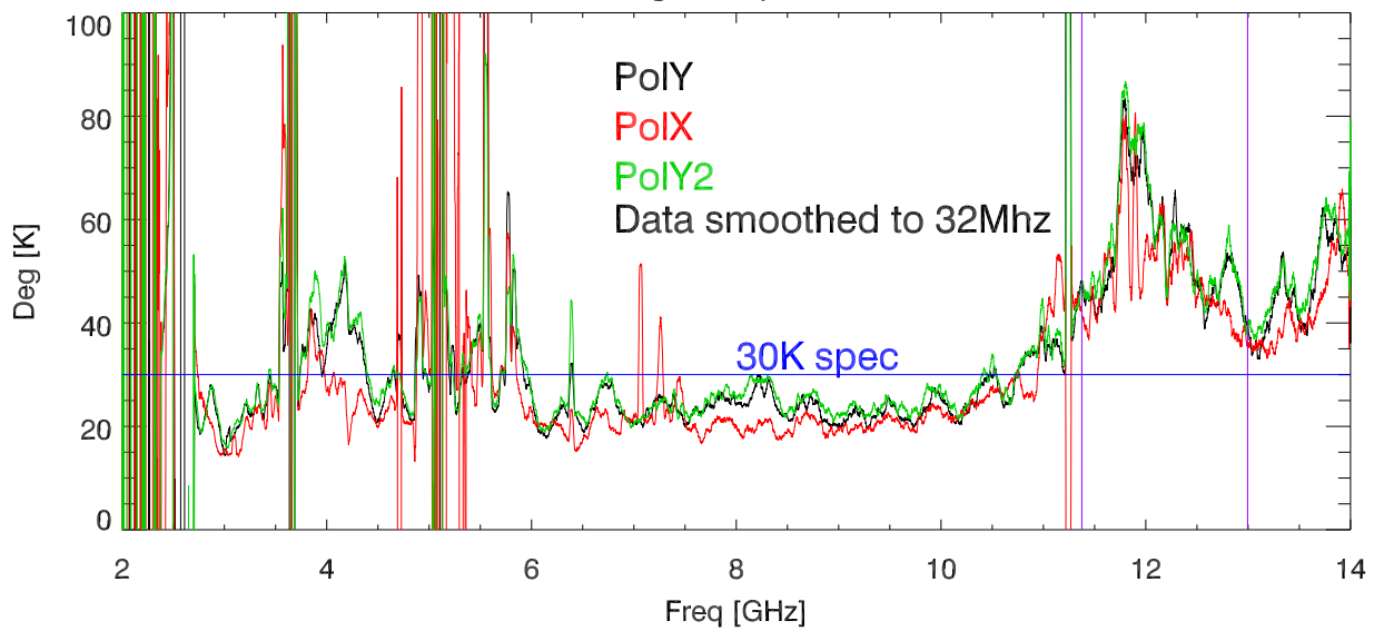
Flange temperature
