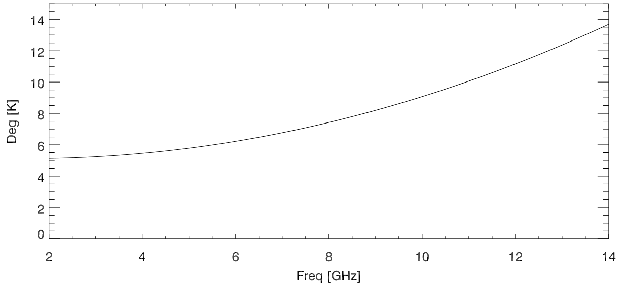
Tsky vs freq (from paulGoldsmiths plot)
