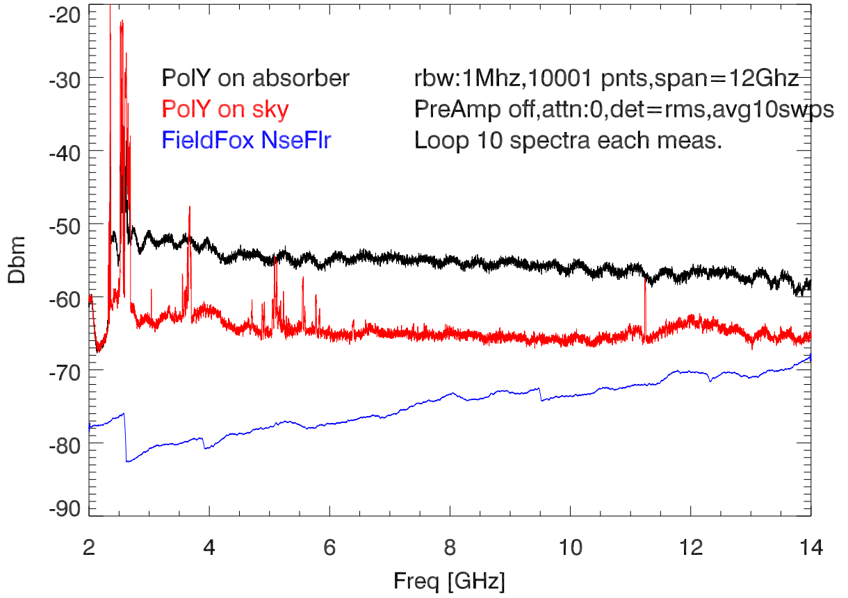
25jan23 wbRcv spectra at test range.
