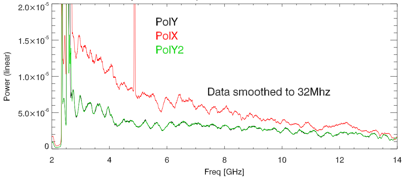
25jan23 cooled qrhf antTestBld. Power on Abs
