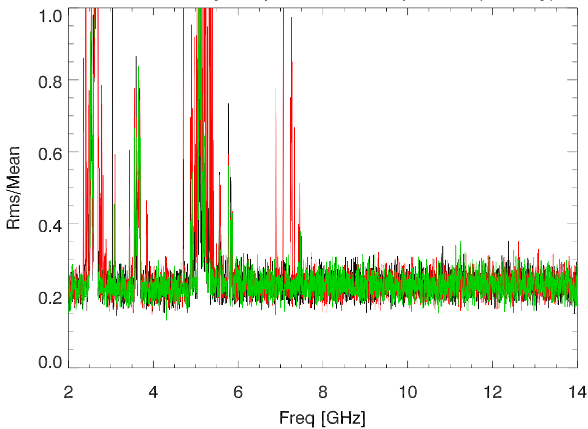
Rms/mean by freq chan for 10 spectra. (on Sky)
