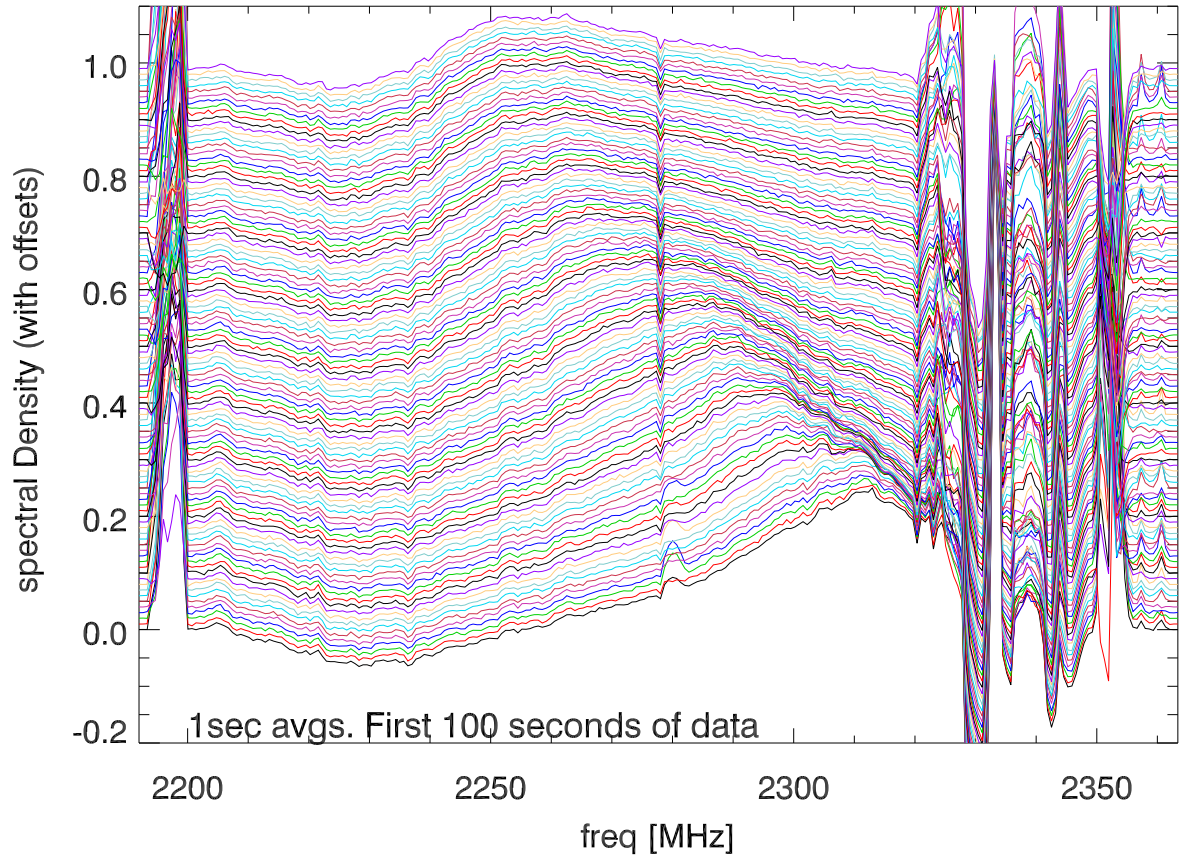
221002 B1641 bandpass corrected spectra with offsets.PoIA
