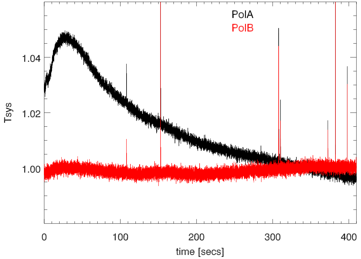
total power vs time (400 secs of file 100)
