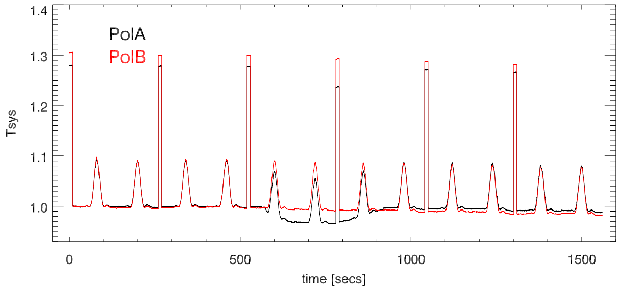
26jun22 xb TotPwr vs time during CasA crosses (8222 MhzBand)
