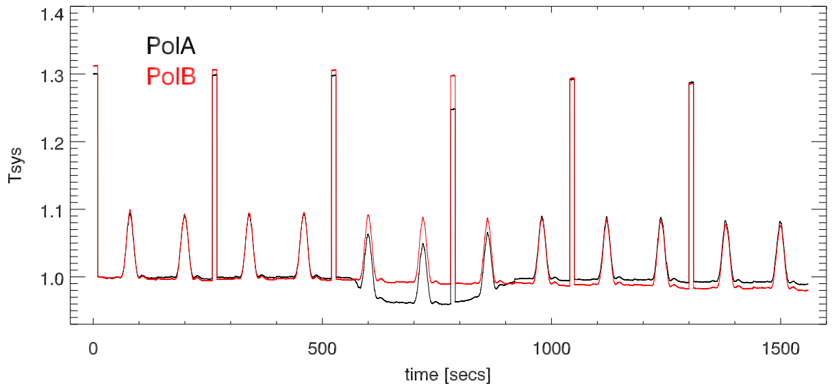
26jun22 xb TotPwr vs time during CasA crosses (8504 MhzBand)
