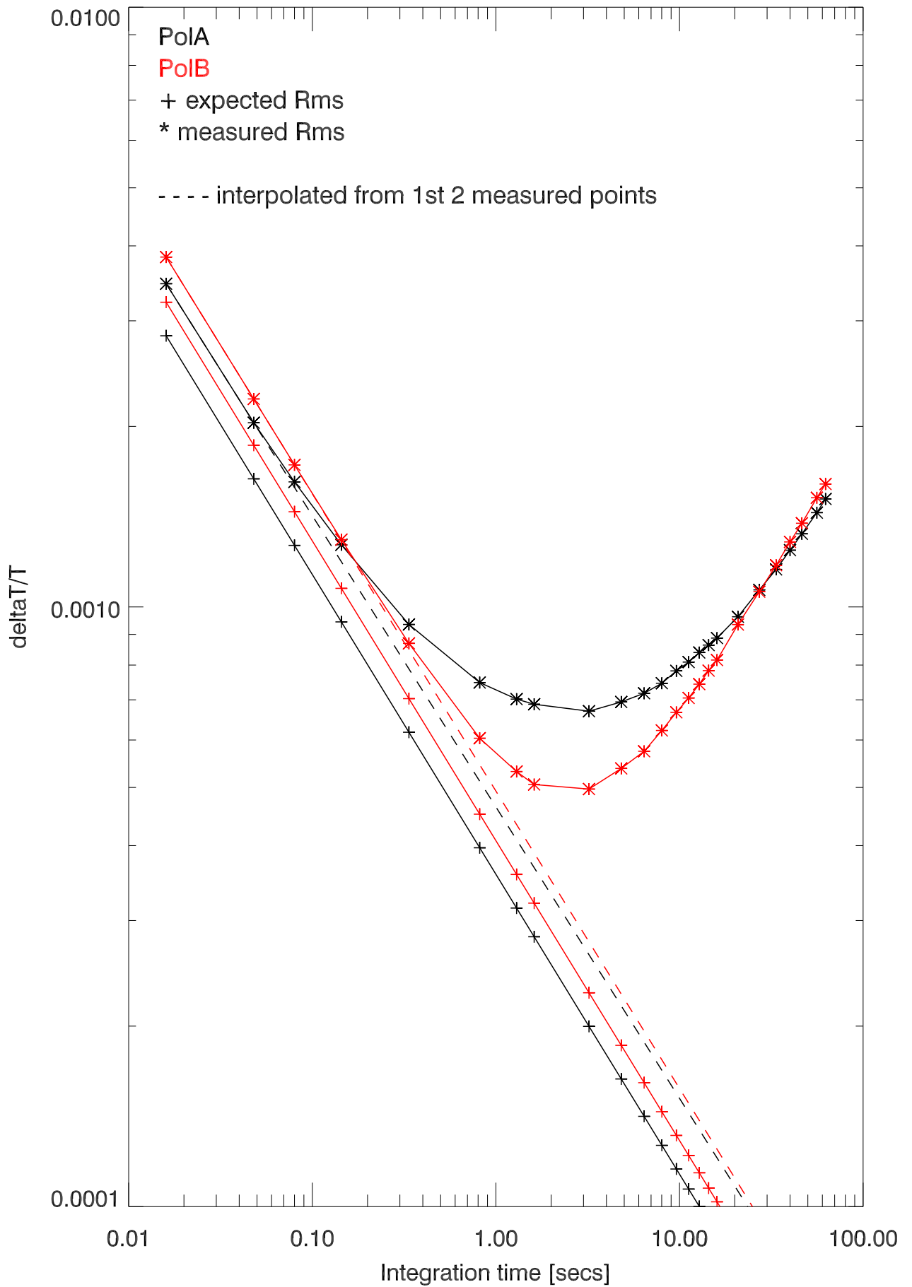
220316 rms Error vs integration time after calCorrection 8219 MHz band
