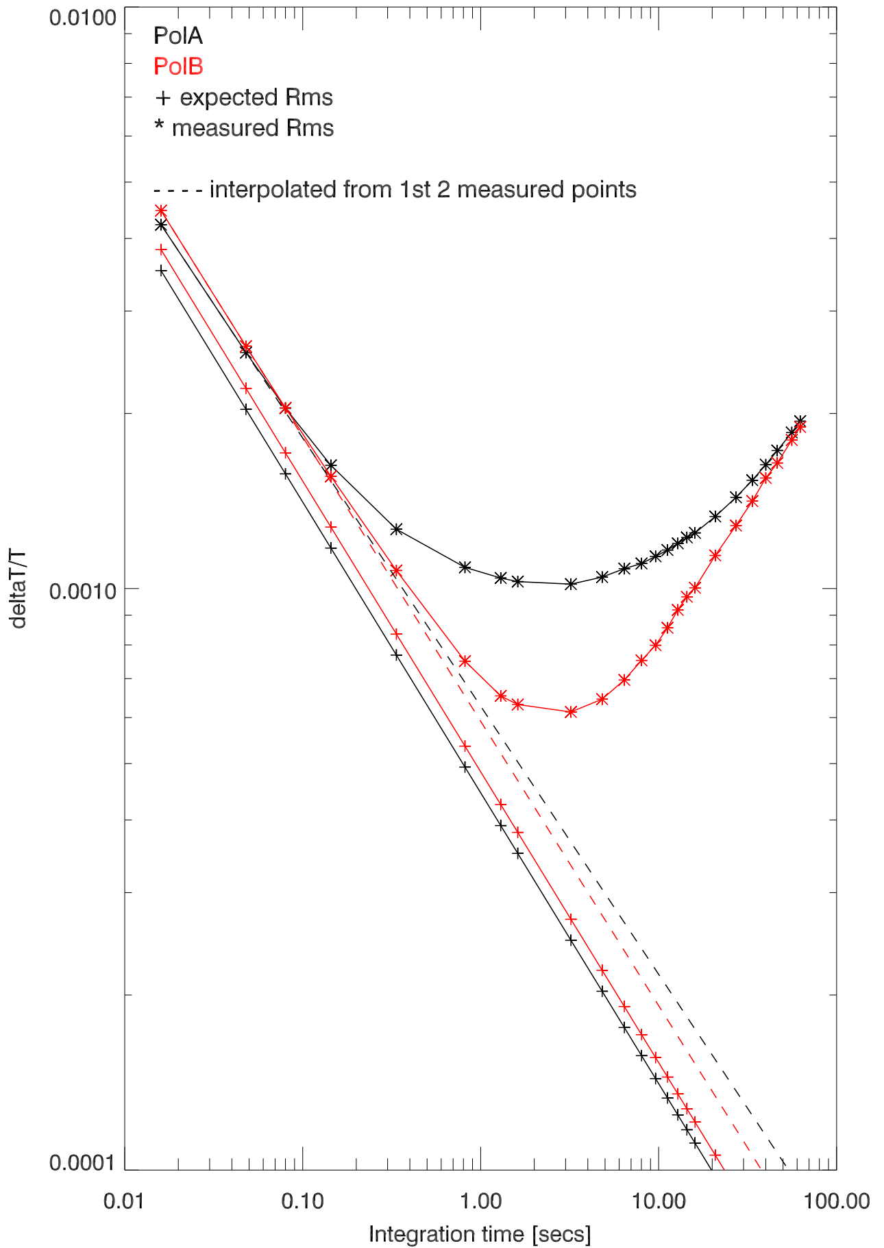
220316 rms Error vs integration time after calCorrection 8931 MHz band
