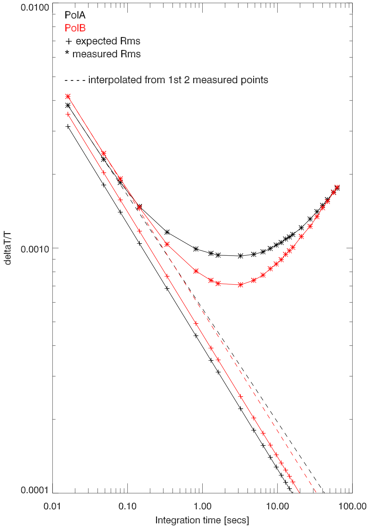
220316 rms Error vs integration time after calCorrection 8789 MHz band
