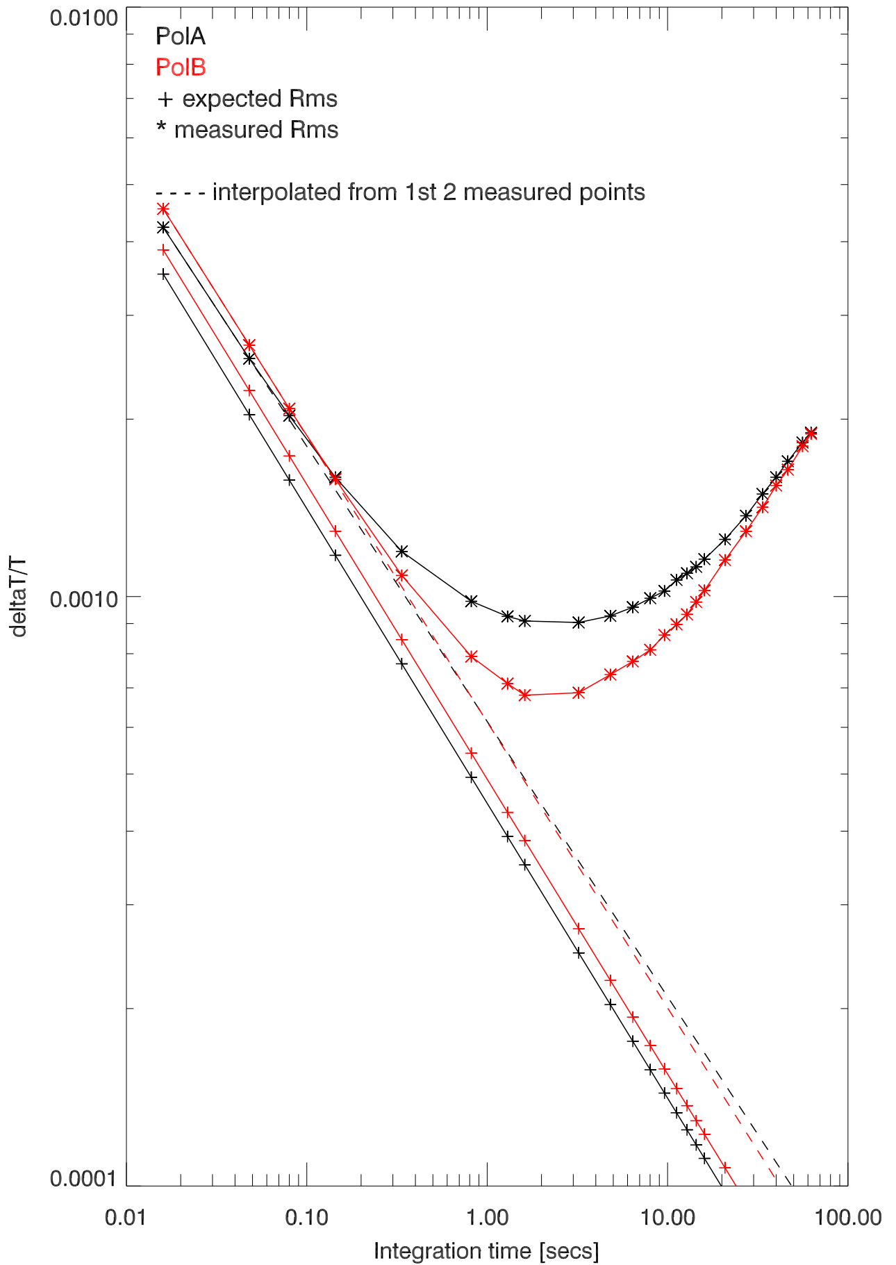
220316 rms Error vs integration time after calCorrection 9073 MHz band
