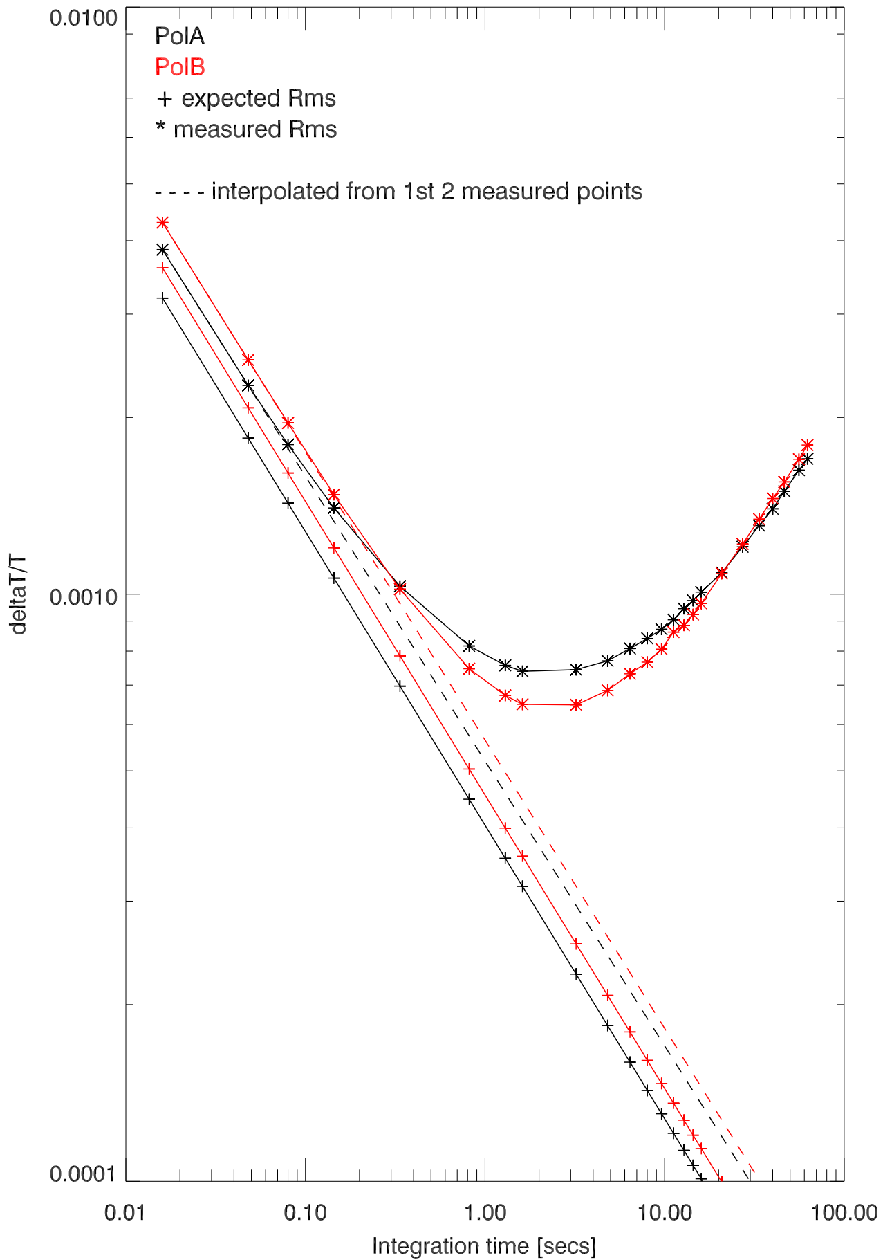
220316 rms Error vs integration time after calCorrection 8363 MHz band
