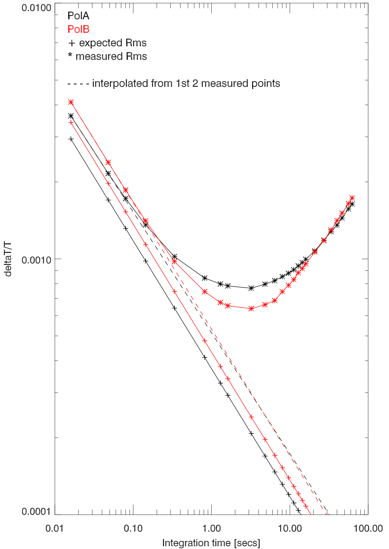
220316 rms Error vs integration time after calCorrection 8505 MHz band
