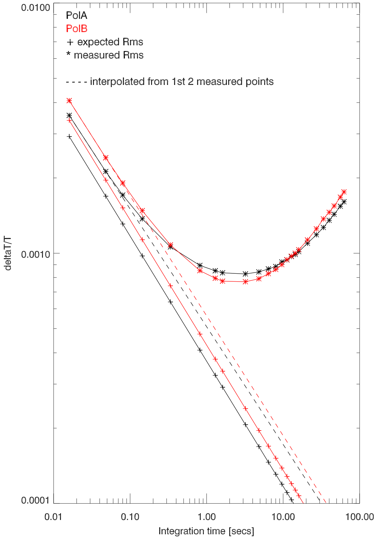
220316 rms Error vs integration time after calCorrection 8647 MHz band
