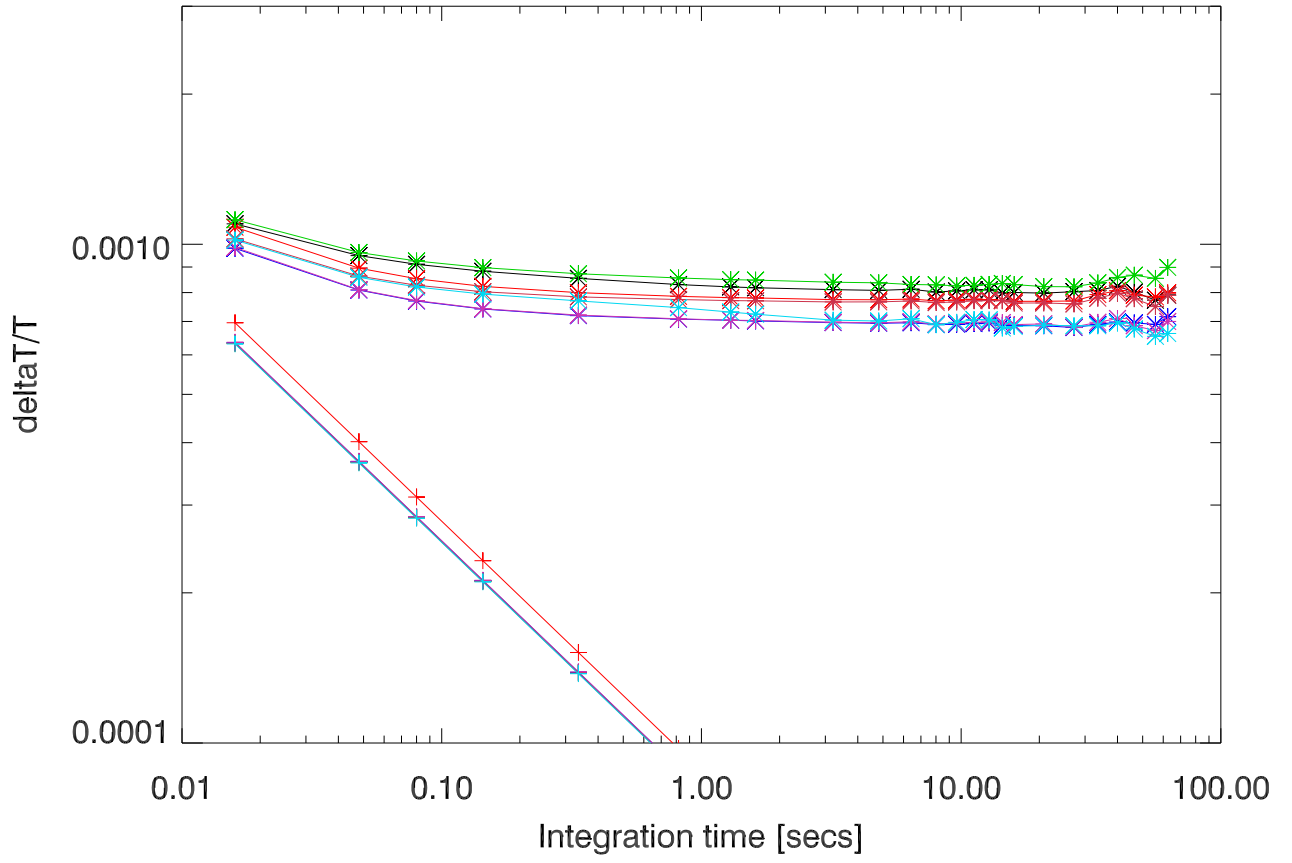
220316 deltaT/T vs integration time no Correction. PoIA
