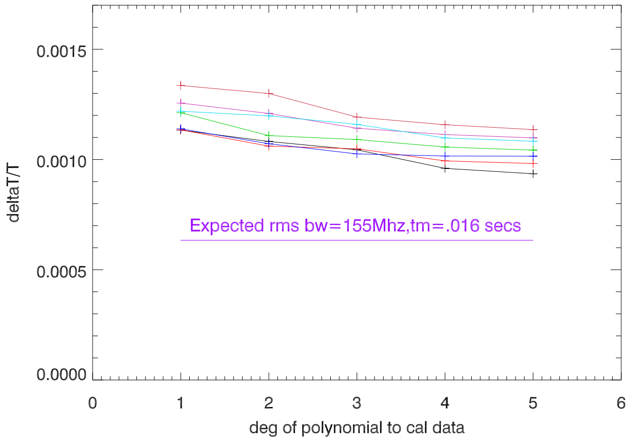
16jan22 RMS of deltaT/T vs Fit order for calDeflection. PoIA
