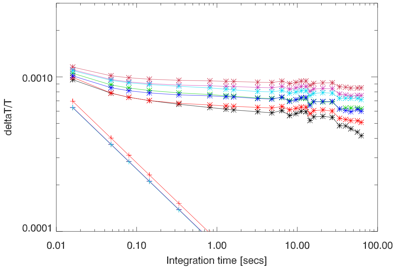
220316 deltaT/T vs integration time corrected with 4th order calFit. PoIA
