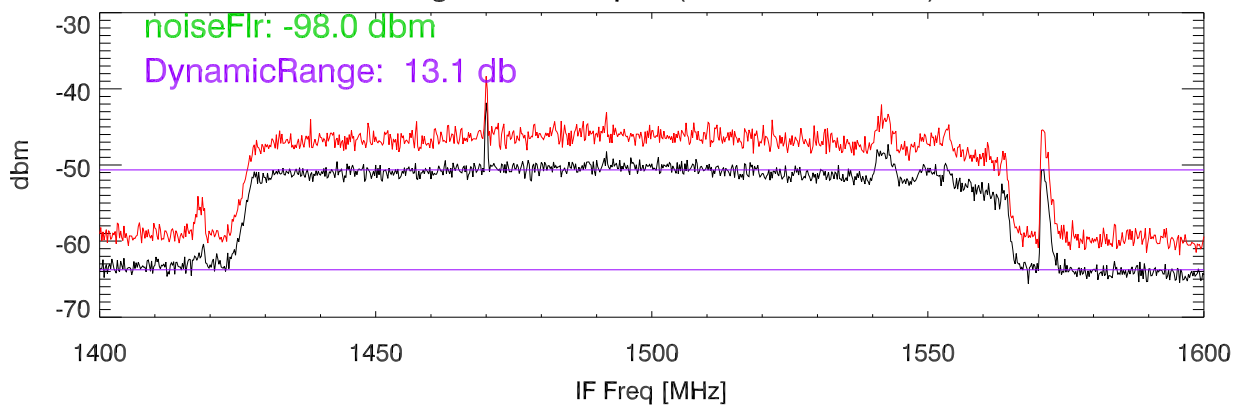
UDC mixing chassis output. (IF 1500=RF 2270). PoIB
