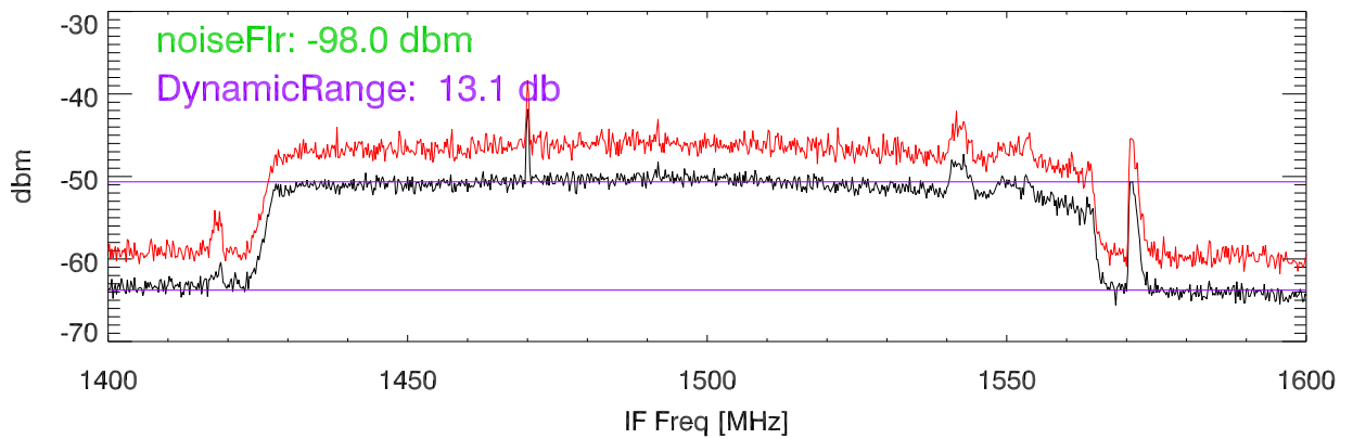
UDC mixing chassis output. (IF 1500=RF 2270). PoIA
