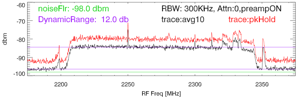
220311 12mSB FOrcvr Output. PoIA
