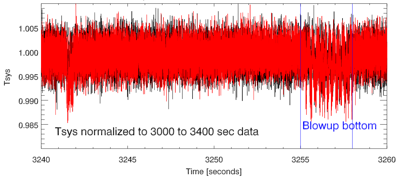
Blowup 3240 to 3260 secs. band=8642 Mhz
