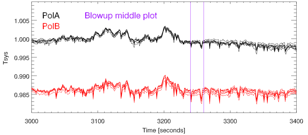
B0329+54 tp vs time: blowup 3000 to 3400 seconds
