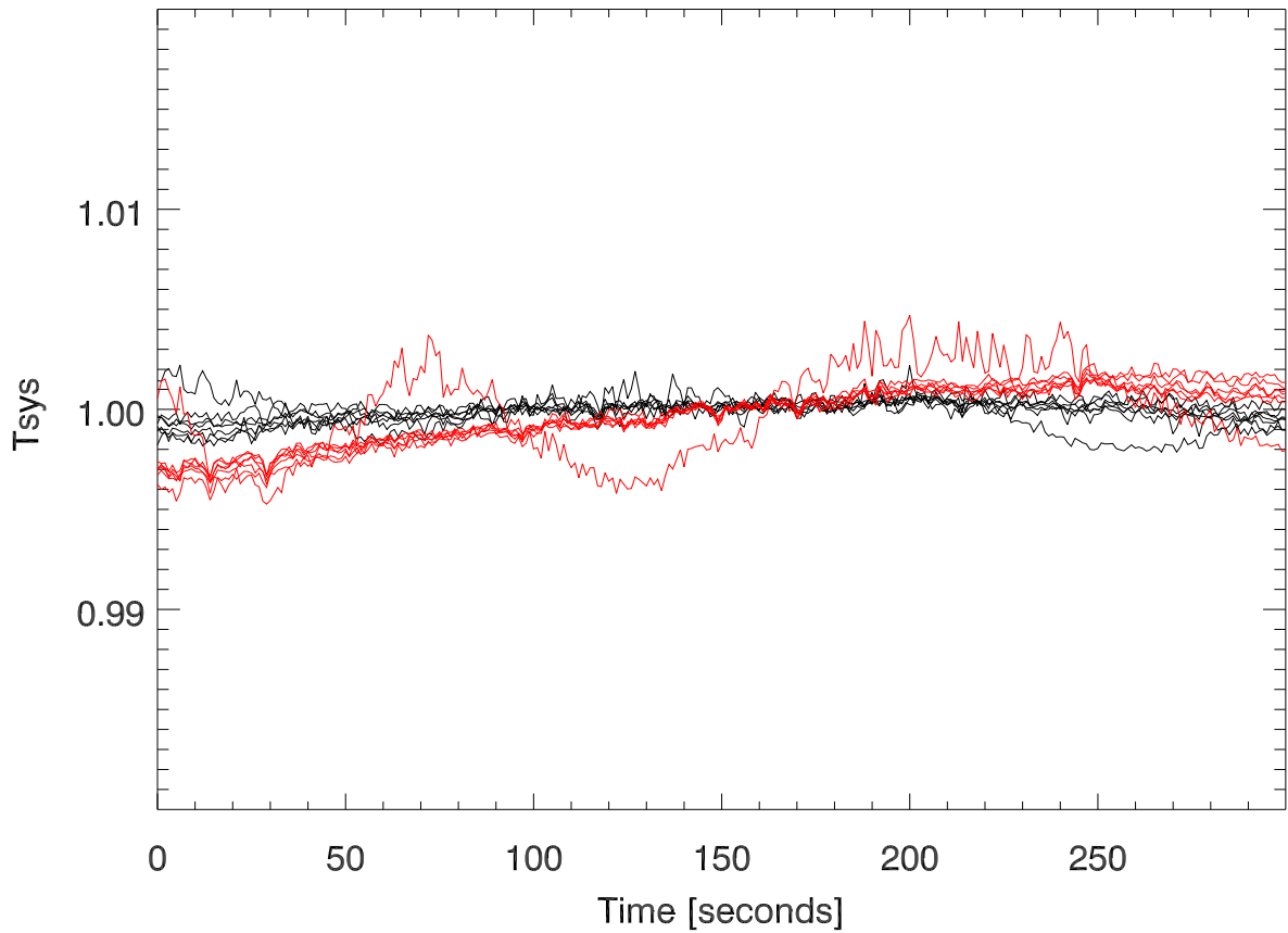
Relative Tsys change vs time for B0833-45
