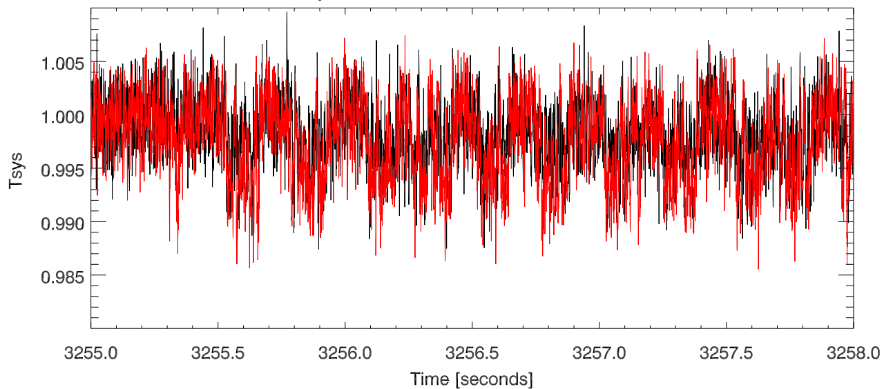
Blowup 3255 to 3258 secs band=8642 Mhz
