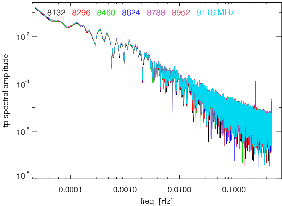
210919 12m xband spectral magnitude of total power. Pol B
