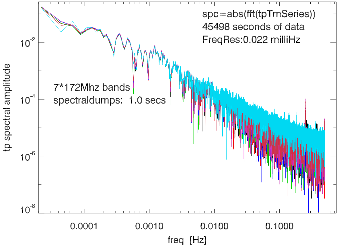
210919 12m xband spectral magnitude of total power. Pol A
