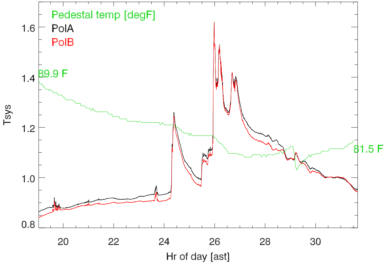
210919 total power vs hour
