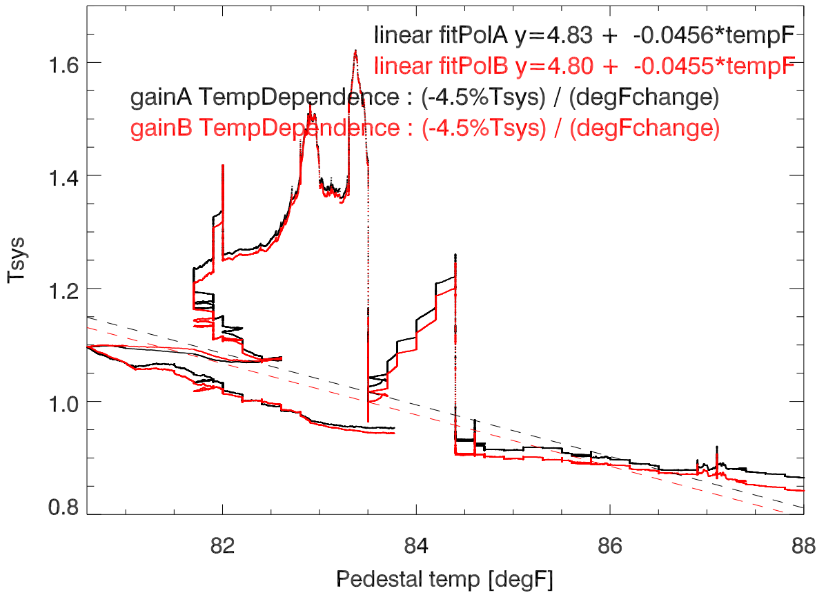
Total power vs pedestal temp
