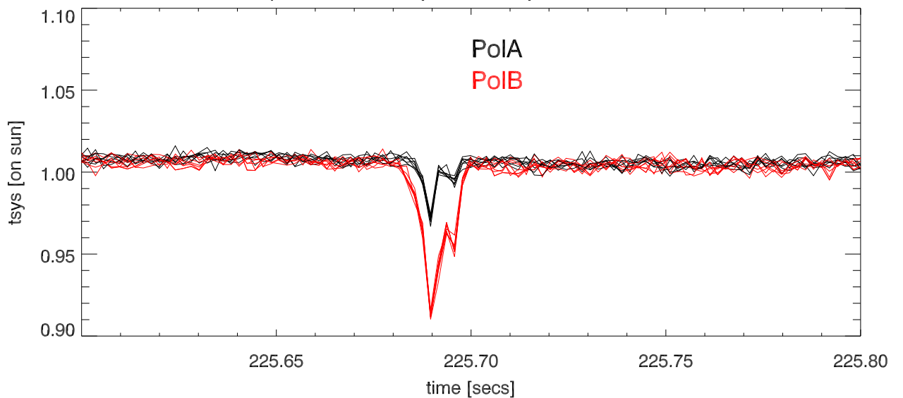
Blowup around 1 dropout. Overplot all 7 bands PoIB
