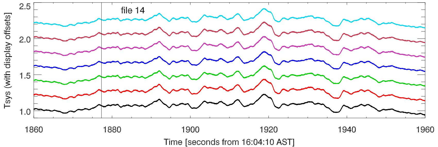
07jul21 12meter xb. totPwr vs time tracking sun. HiRes PoIB
