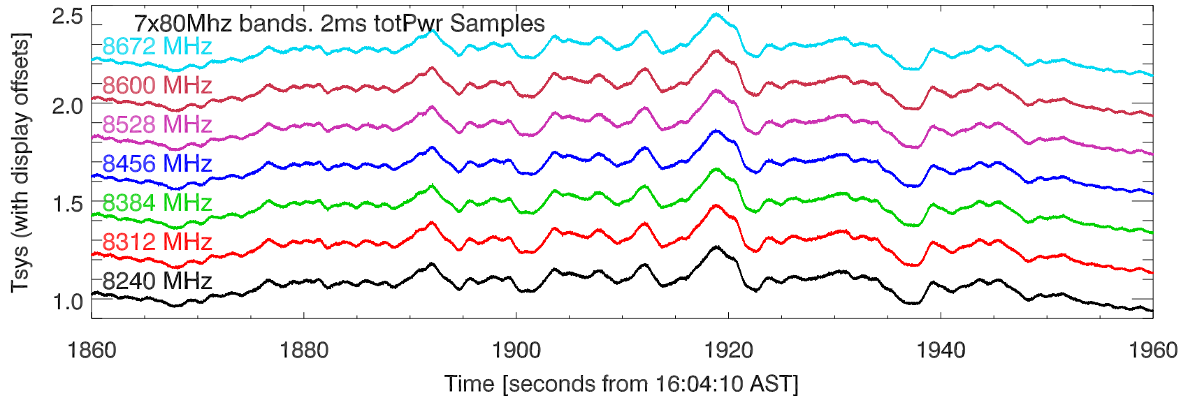
07jul21 12meter xb. totPwr vs time tracking sun. HiRes PoIA
