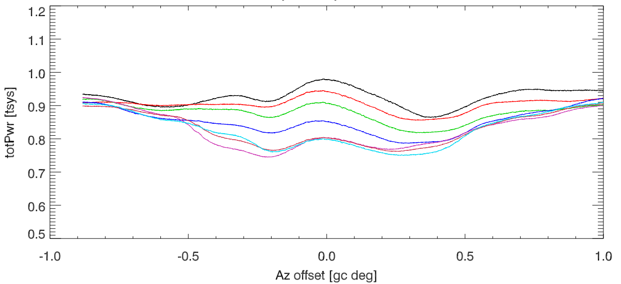
tpPoIA/tpPoIB
