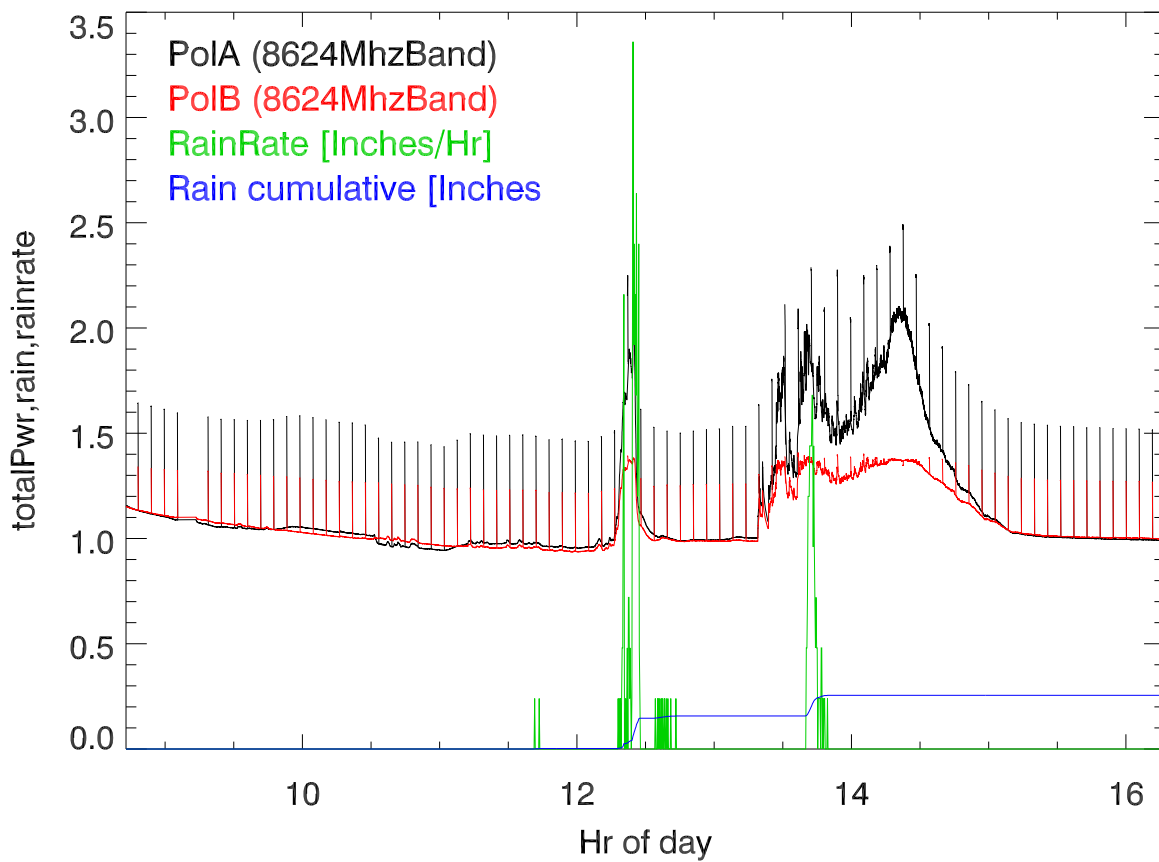
totPwr (8624Mhz) vs hr and rain/rainrate
