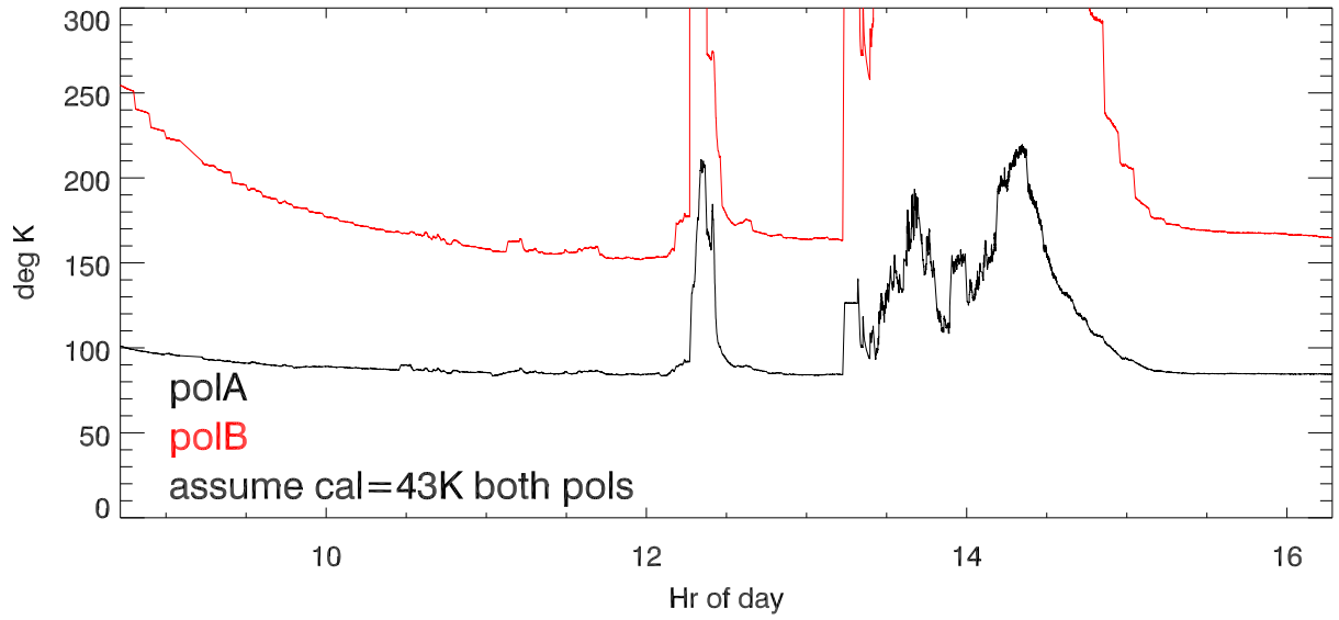
8jun21 p12m xb Tsys vs Hr (using cal deflection)
