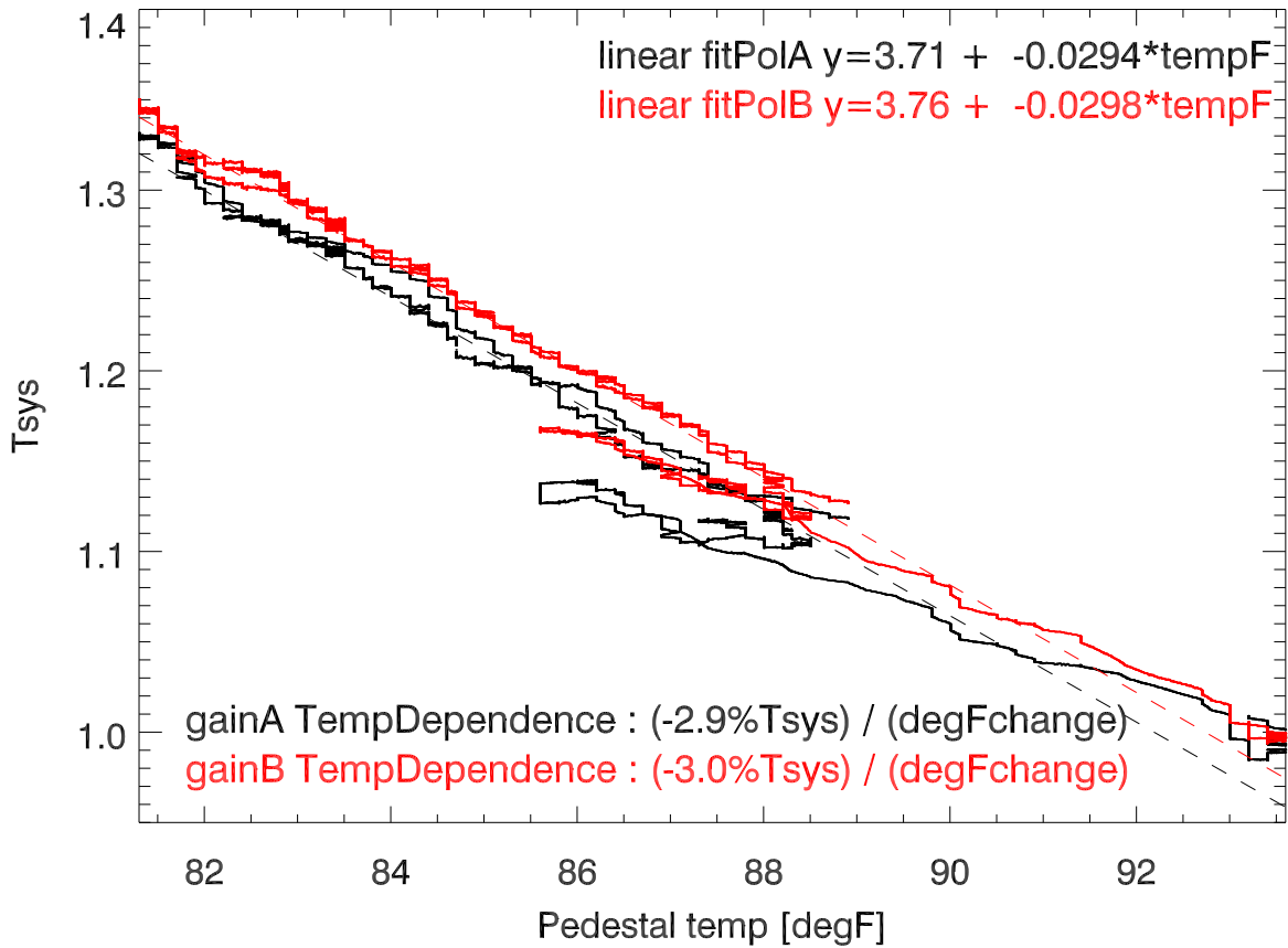
Total power vs pedestal temp
