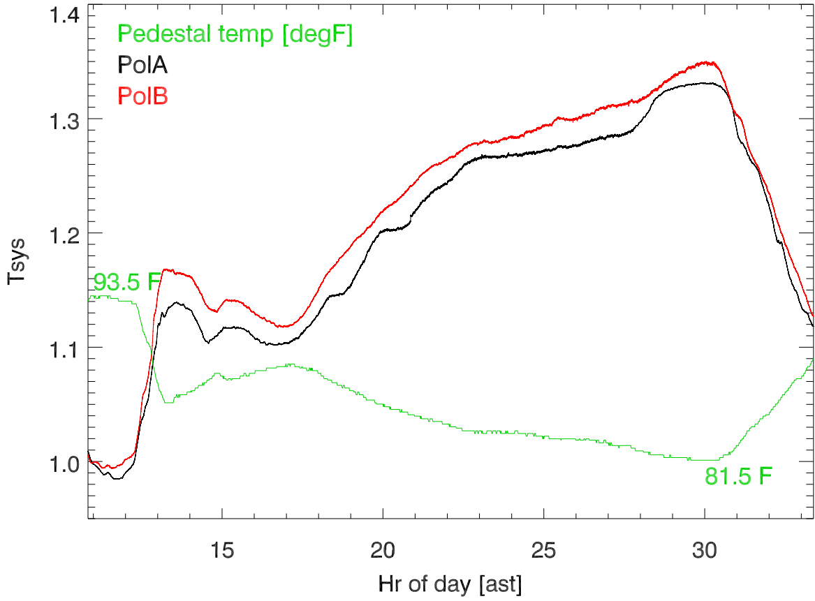
210601 total power vs hour
