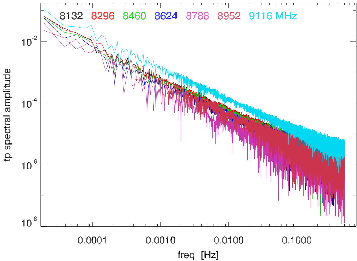
210430 12m xband spectral magnitude of total power. Pol B
