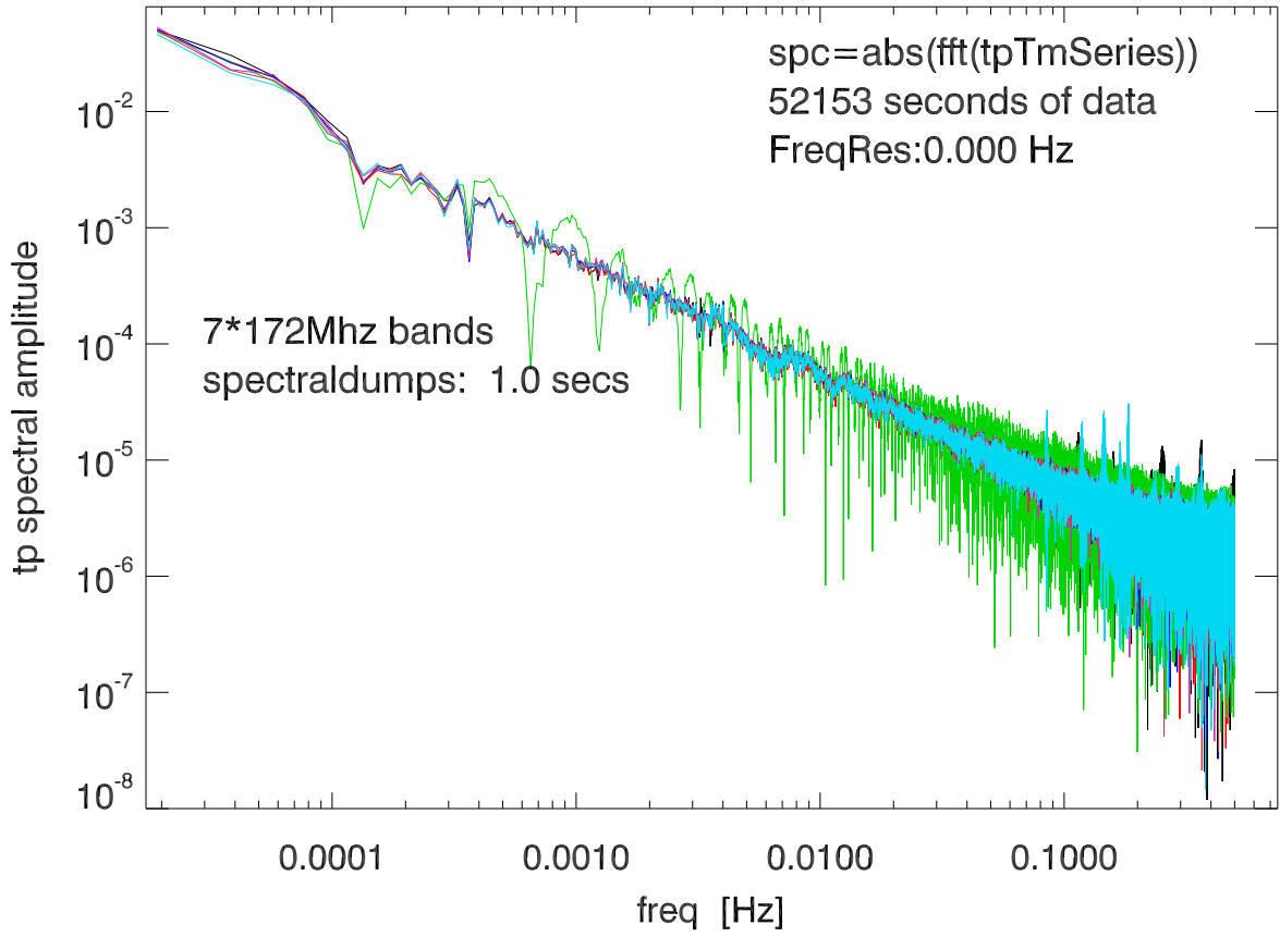
210430 12m xband spectral magnitude of total power. Pol A
