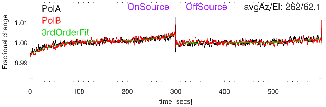
220819 3C274 Fractional change cal Deflection vs time. BandCfr:8219.0 Pat:1
