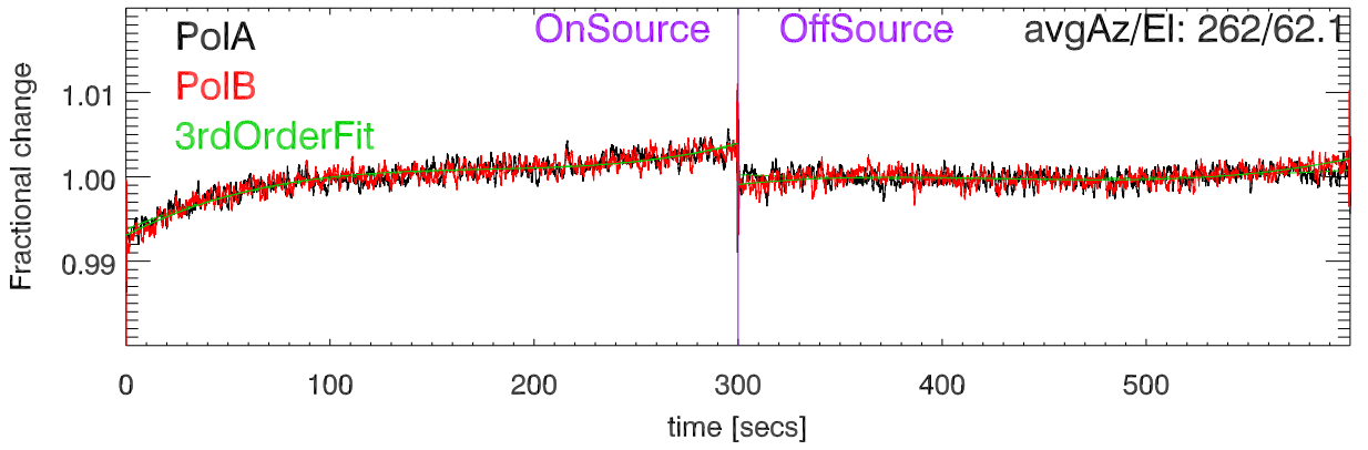
220819 3C274 Fractional change cal Deflection vs time. BandCfr:8647.0 Pat:1
