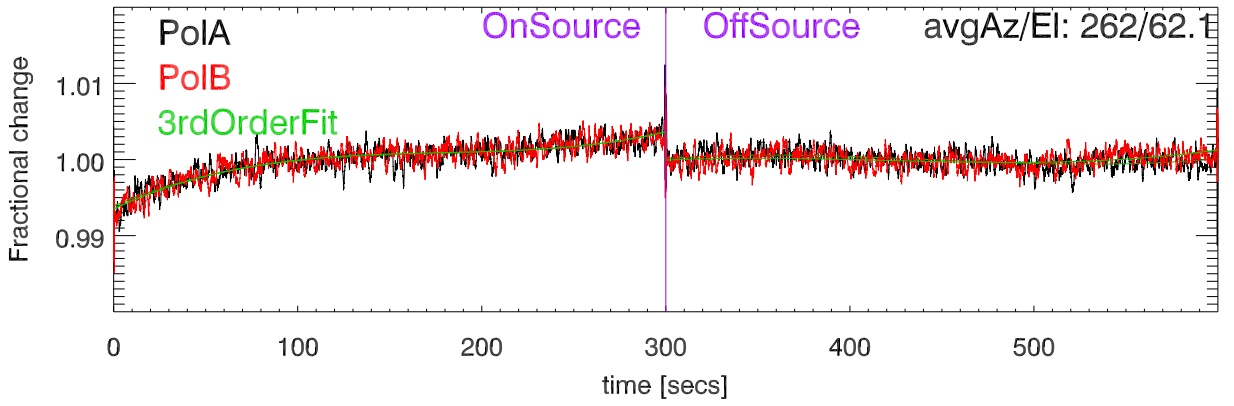
220819 3C274 Fractional change cal Deflection vs time. BandCfr:8931.0 Pat:1
