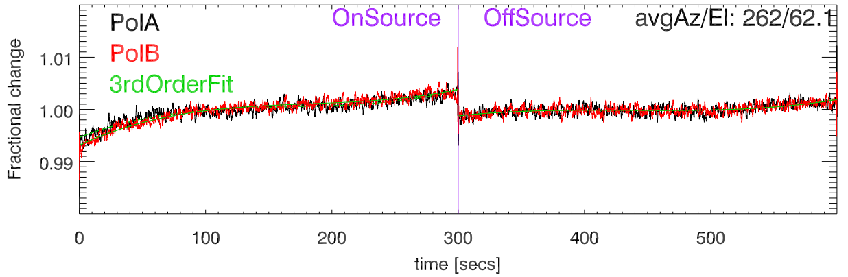
220819 3C274 Fractional change cal Deflection vs time. BandCfr:8363.0 Pat:1
