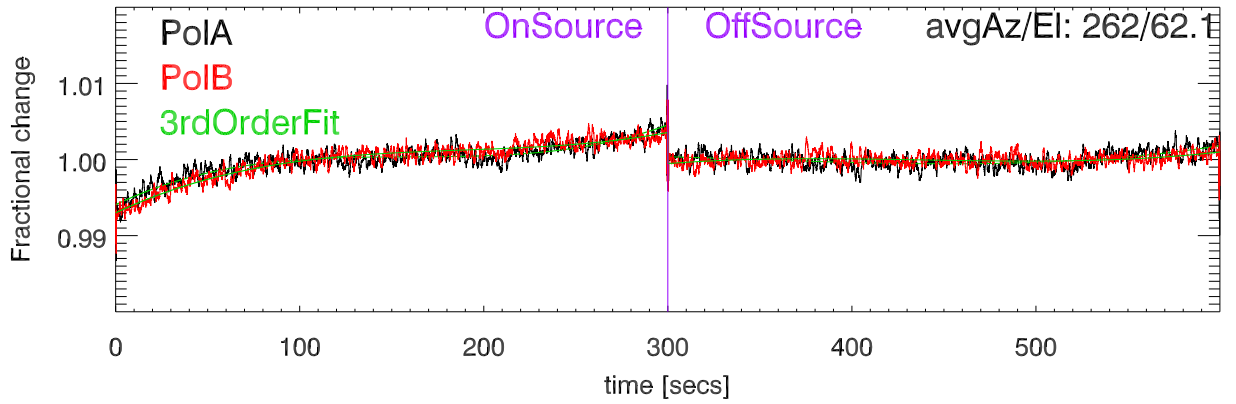
220819 3C274 Fractional change cal Deflection vs time. BandCfr:8505.0 Pat:1
