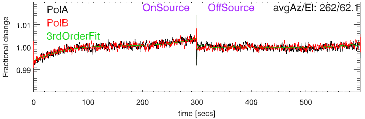
220819 3C274 Fractional change cal Deflection vs time. BandCfr:8789.0 Pat:1
