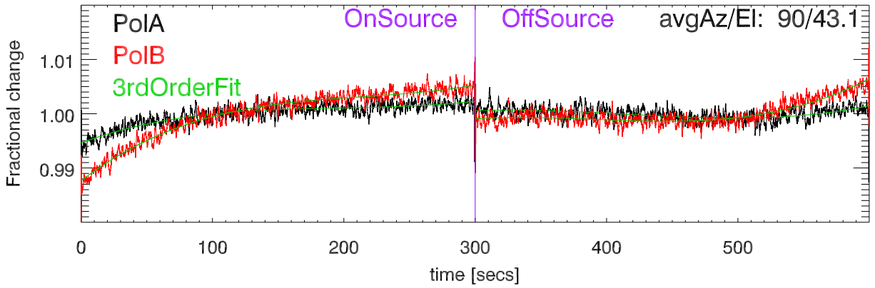
220803 3C274 Fractional change cal Deflection vs time. BandCfr:8789.0 Pat:1
