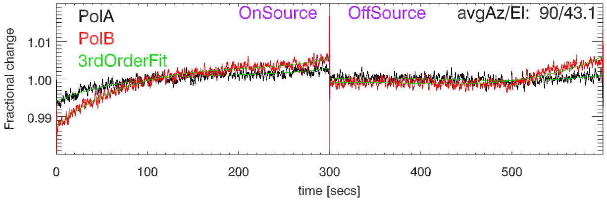
220803 3C274 Fractional change cal Deflection vs time. BandCfr:8647.0 Pat:1
