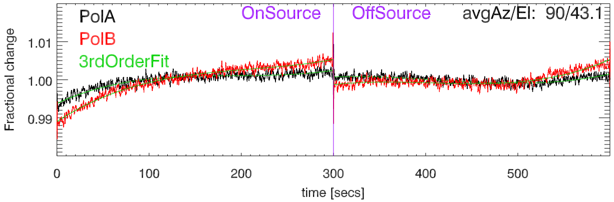
220803 3C274 Fractional change cal Deflection vs time. BandCfr:8505.0 Pat:1
