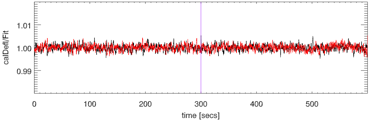
CalDeflection/Fit: fractional gain variation after correction
