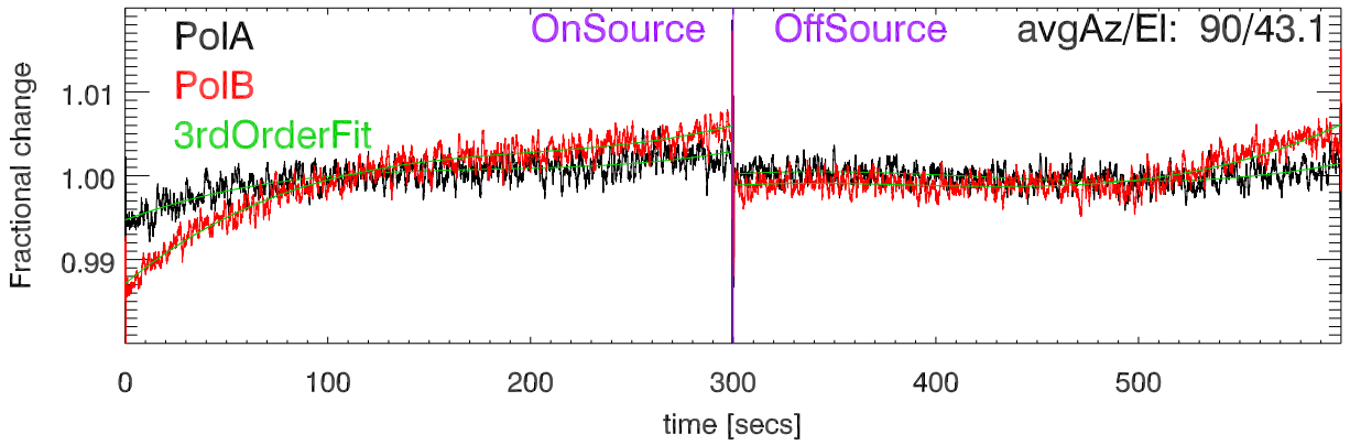
220803 3C274 Fractional change cal Deflection vs time. BandCfr:8931.0 Pat:1
