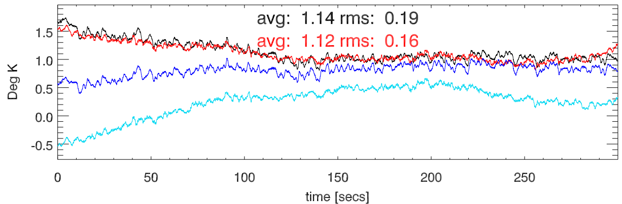
SrcDeflection vs time (calOff)
