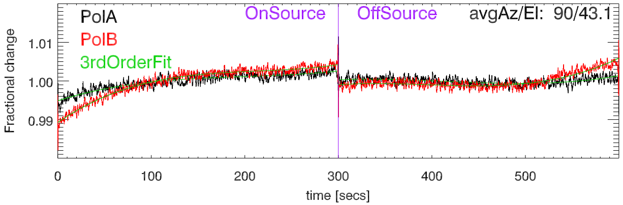
220803 3C274 Fractional change cal Deflection vs time. BandCfr:8219.0 Pat:1
