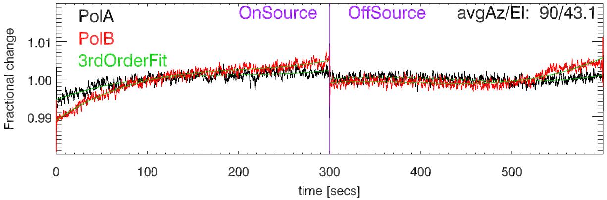
220803 3C274 Fractional change cal Deflection vs time. BandCfr:8363.0 Pat:1
