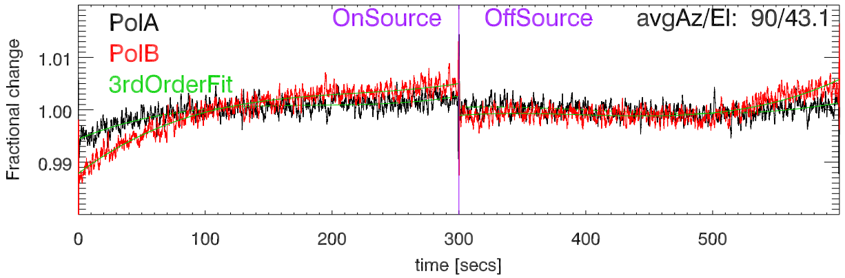
220803 3C274 Fractional change cal Deflection vs time. BandCfr:9073.0 Pat:1
