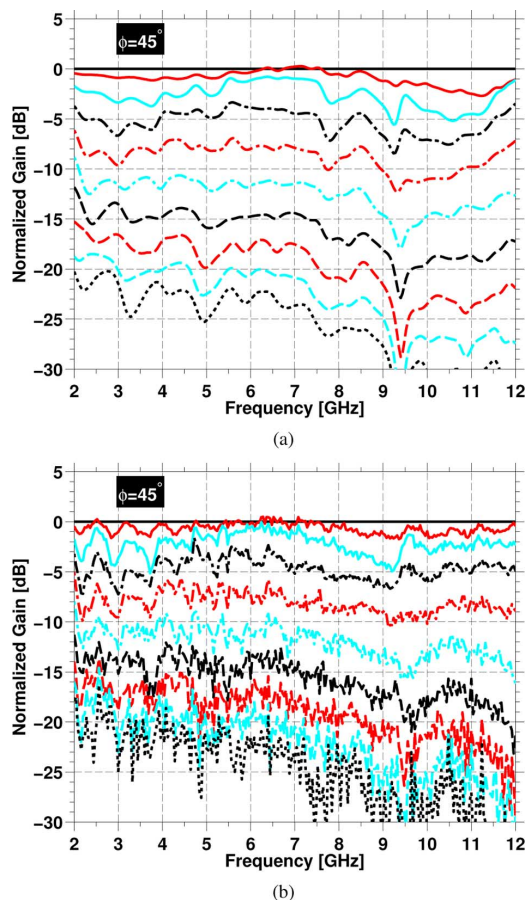
Fig. 10. (a) Simulated and (b) measured gain versus frequency at \theta angles from 0^\circ to 90^\circ in steps of 10^\circ . The curves are at \phi = 45^\circ and are normalized to \theta = 0^\circ .
