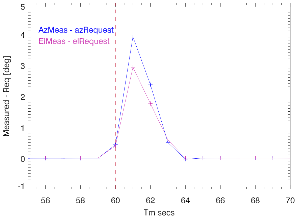
Blowup (Measured - Requested) positions during cross
