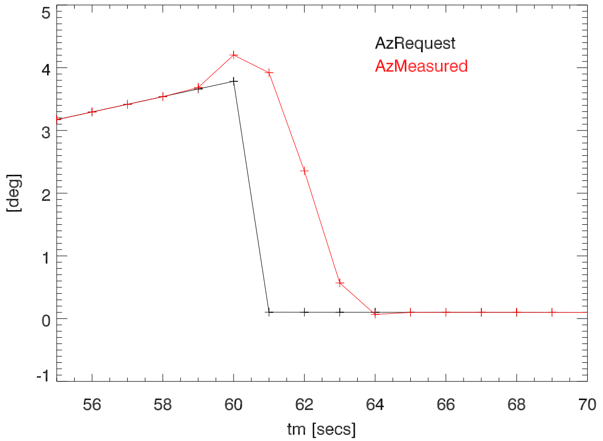
az Req and measured position(remove mean)
