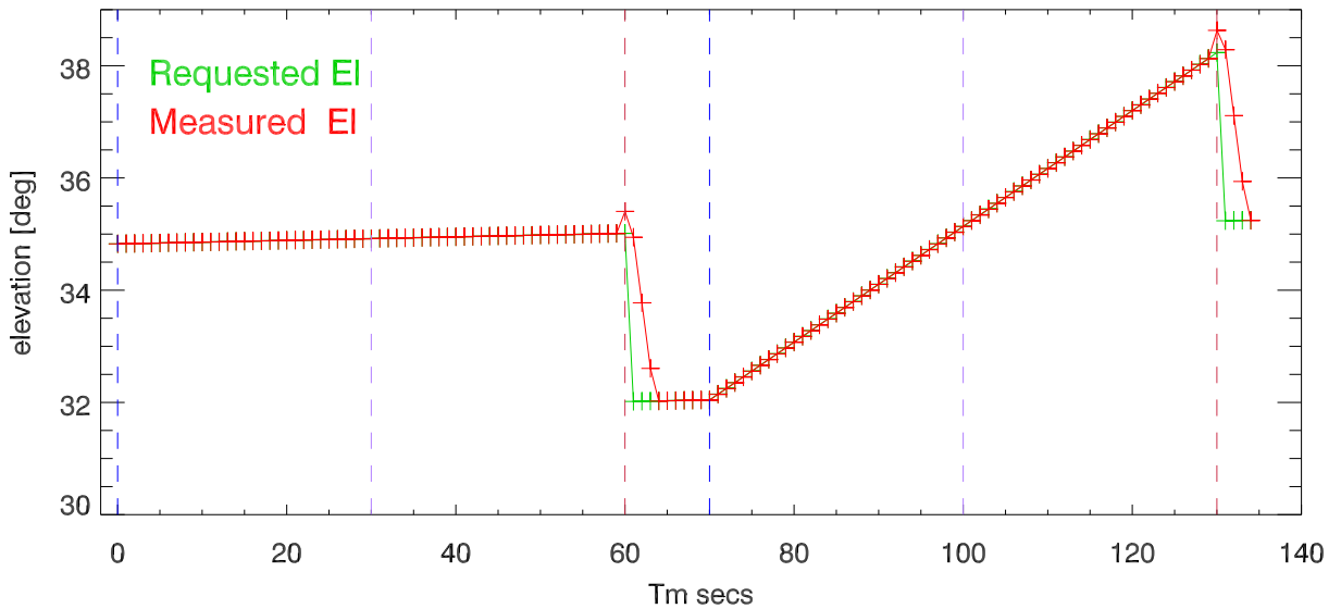
Requested and measured elevation positions
