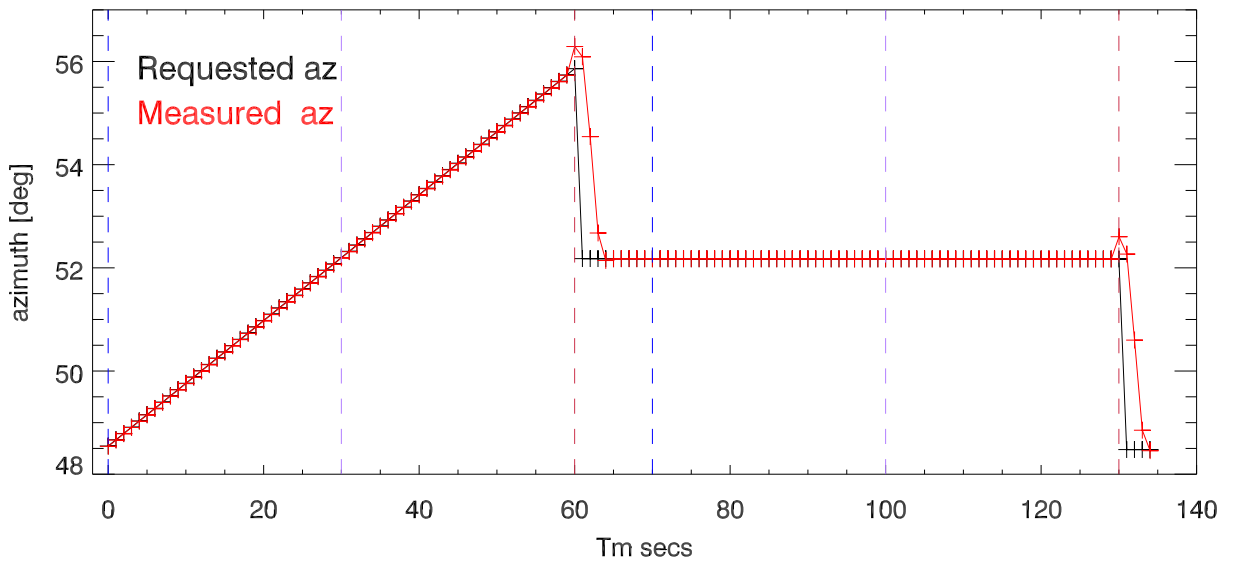
Requested and measured Azimuth positions
