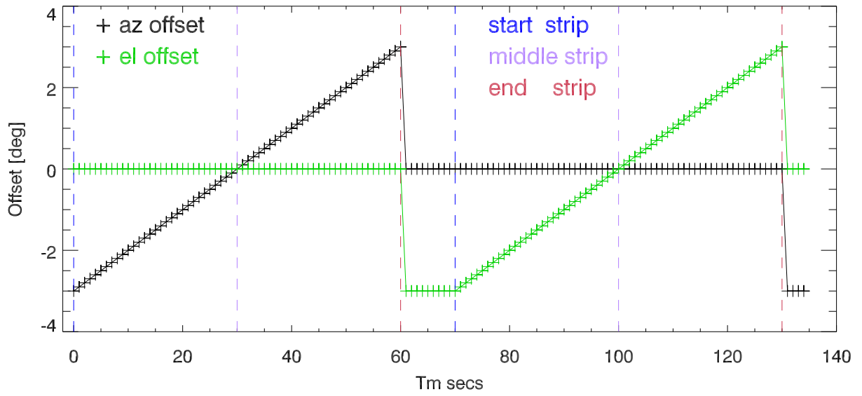
(1dec14) 12m Cross with TrkArr. az,el Req offsets (+/- 3deg @ .1deg/sec)
