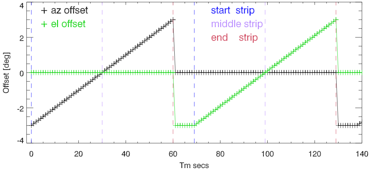
(04dec14) 12m Cross with Ramps. az,el Req offsets (+/- 3deg @ .1deg/sec)
