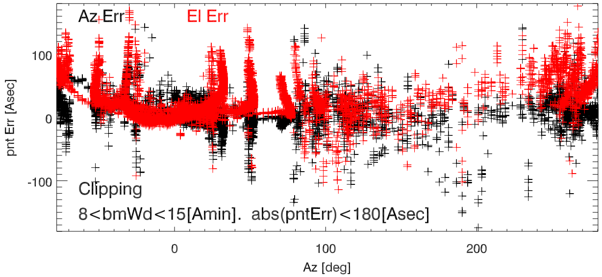
Az,El pnt error vs azimuth (all Freq). Old model Not removed
