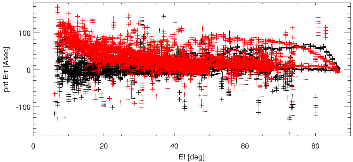
Az,El pnt error vs elevation (all Freq)
