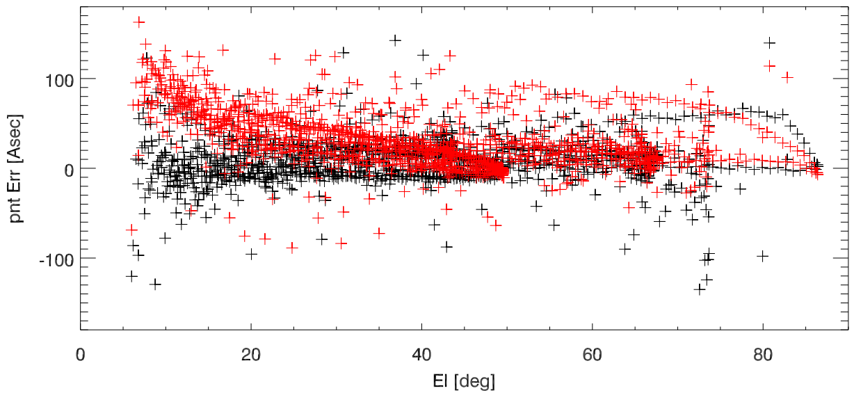
Pnt error vs elevation. (using median value of freqs)
