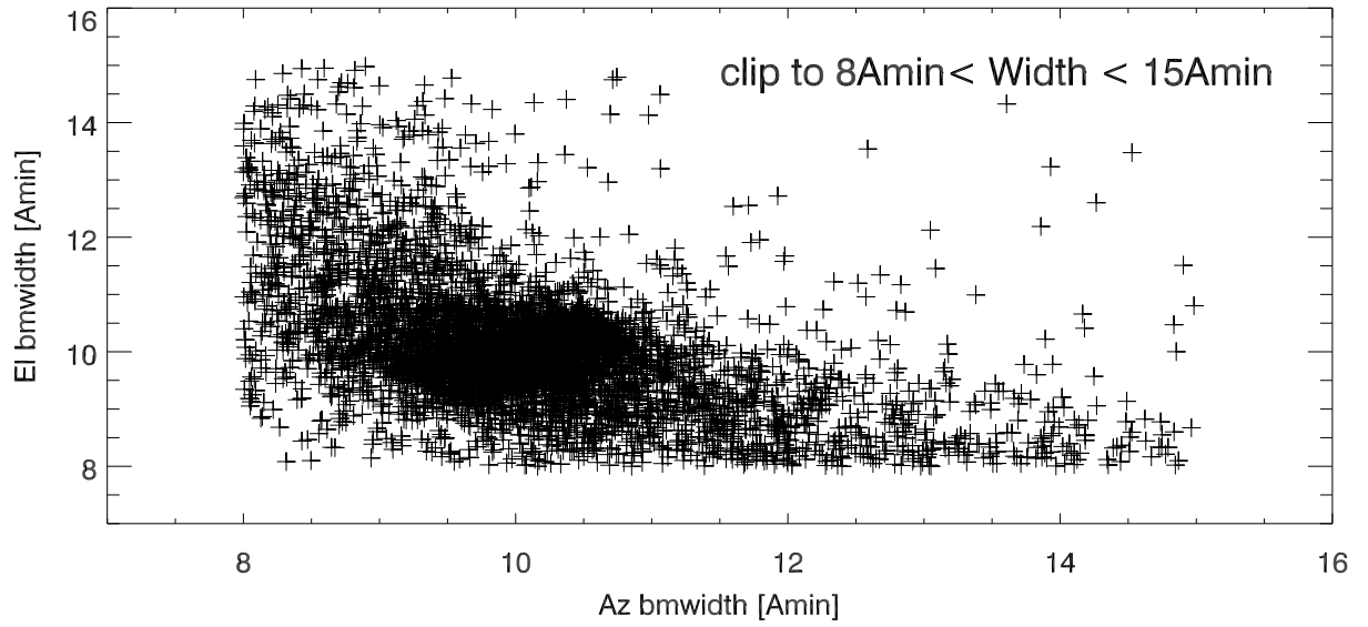
Jul21 Elevation vs Azimuth bmWidths from 2d fits. (All Freqs)
