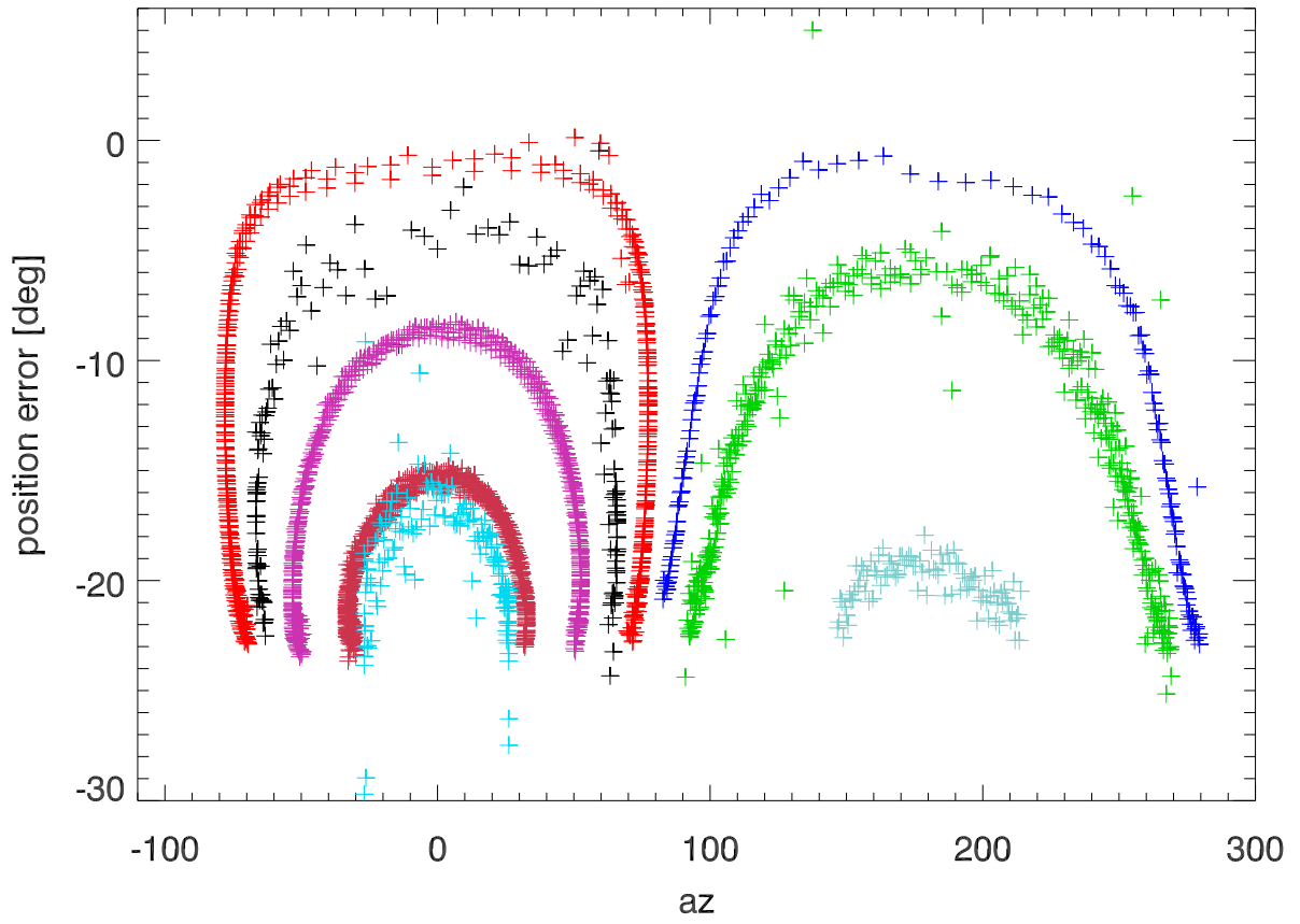
az position errors (GC) vs azimuth [model removed]
