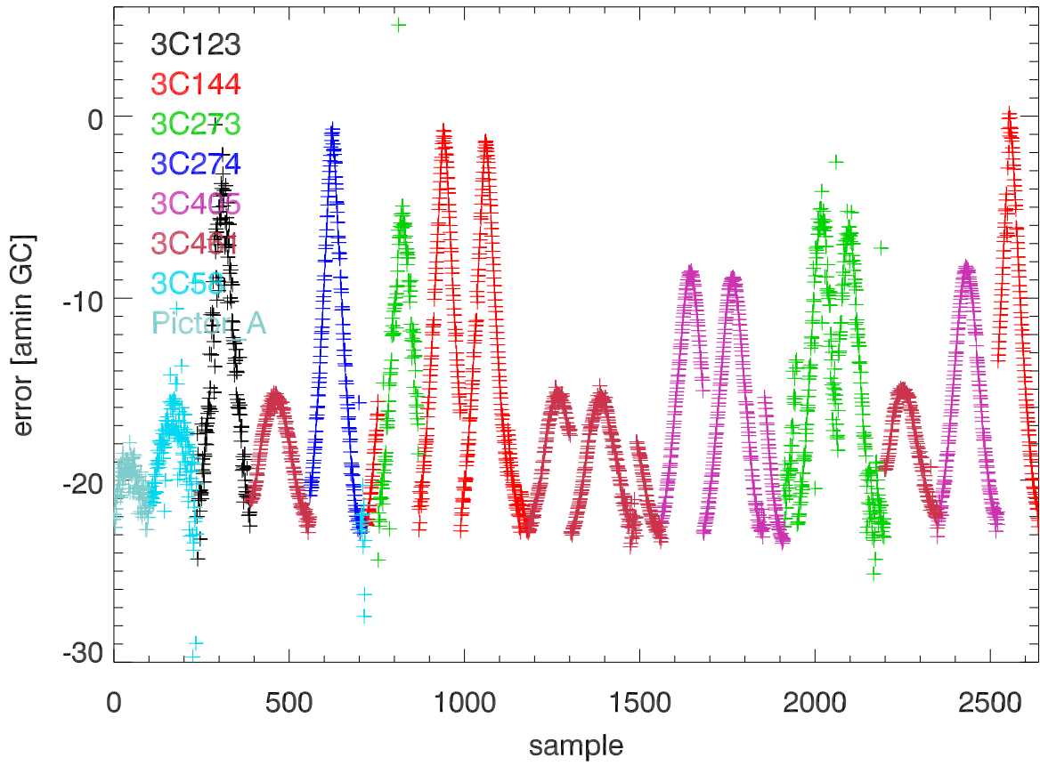
raw az Errs vs sample [old model removed]
