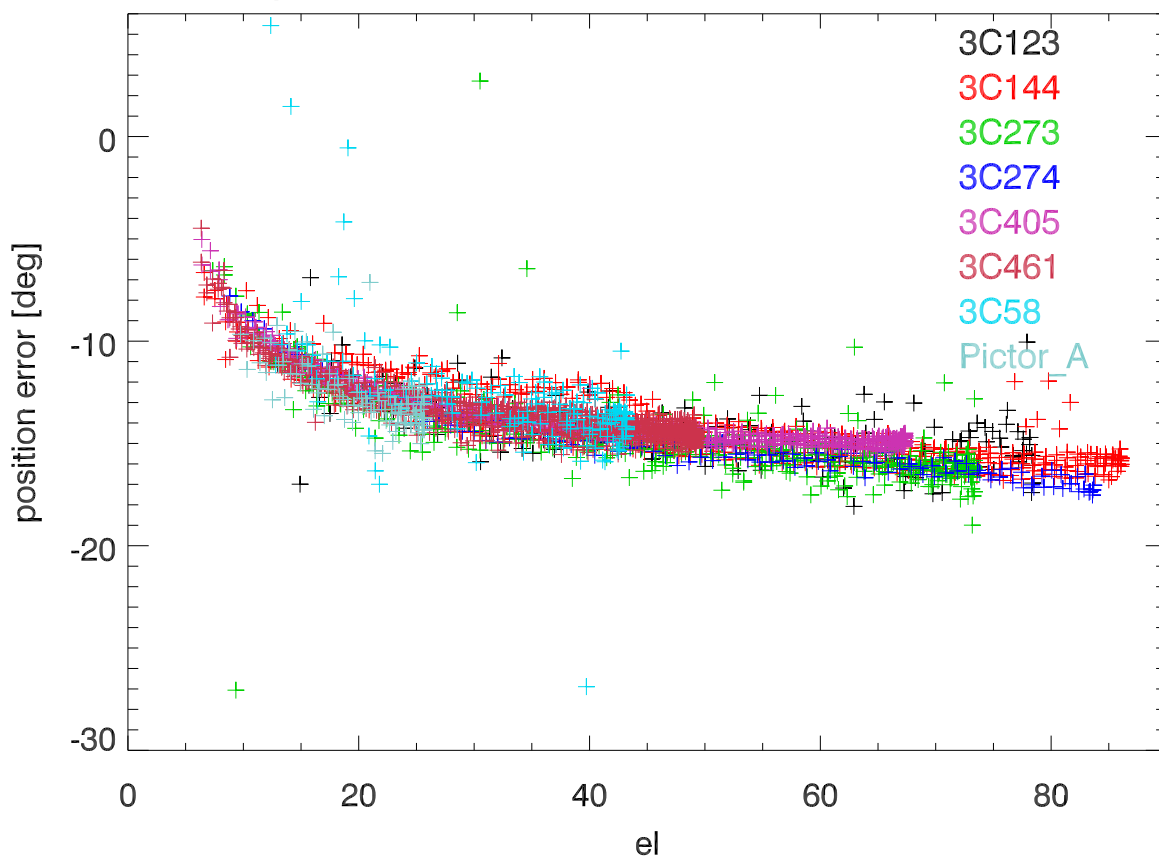
el position errors (GC) vs el [model removed]
