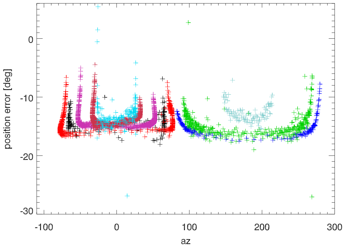
el position errors (GC) vs azimuth [model removed]
