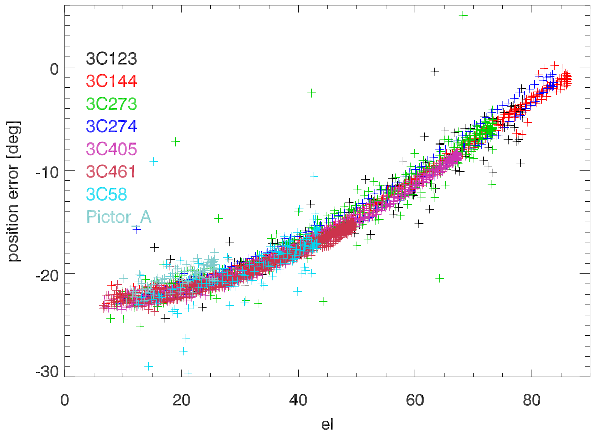
az position errors (GC) vs el [model removed]
