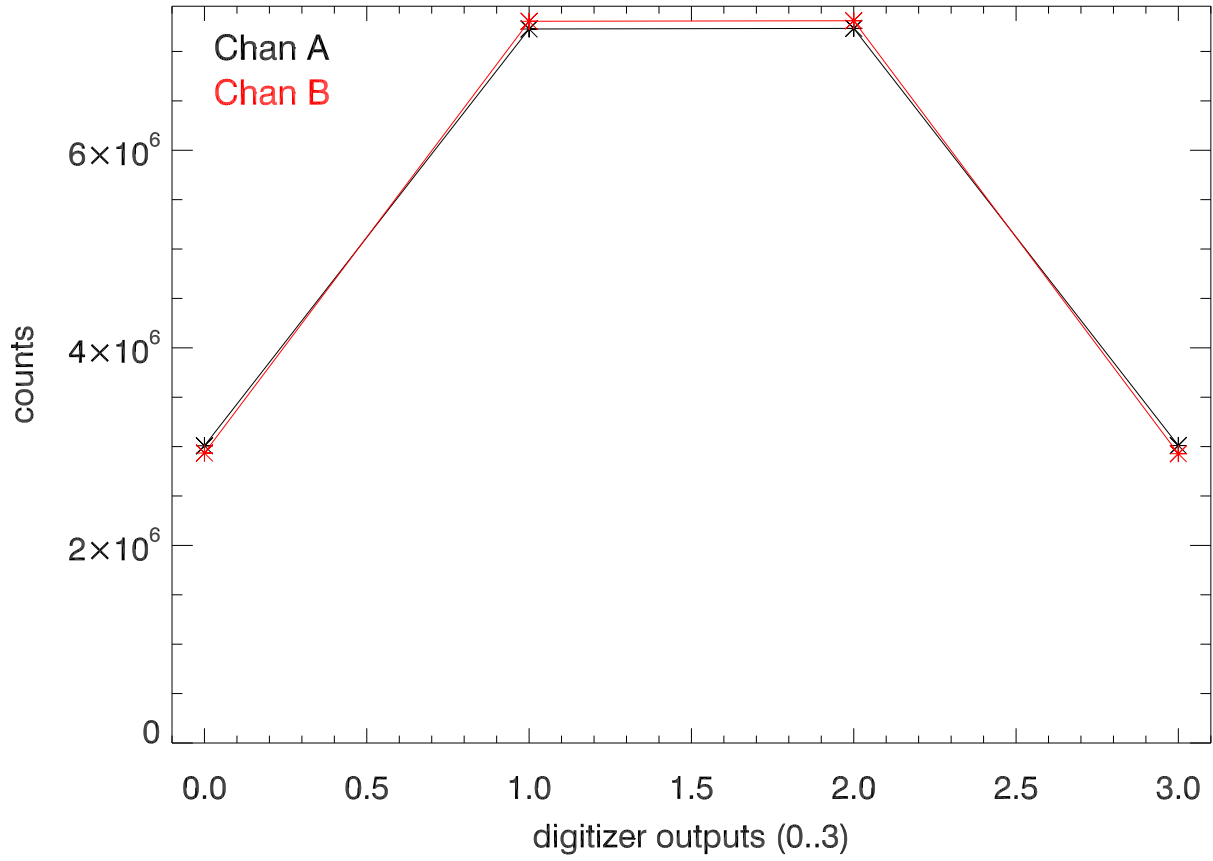
histogram of 2bit raw a/d outputs. t003aa
