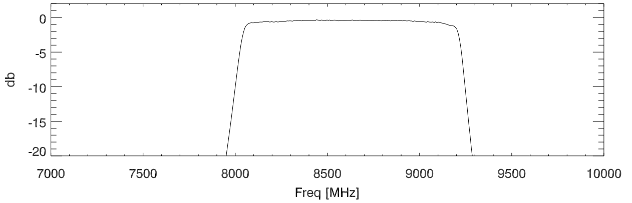
230503: S-parameters for 8.625Ghz_bp. S21
