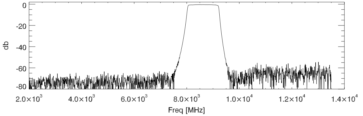
230503: S-parameters for 8.625Ghz_bp. S21
