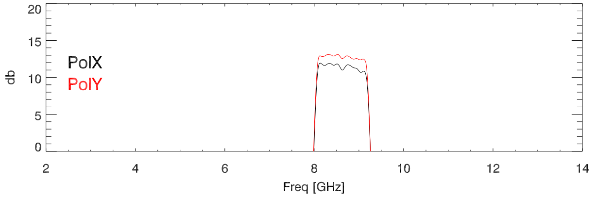
FilterBox Sparams. filtNum=6, cfr=8625 (8037-9213) bandpass. S21
