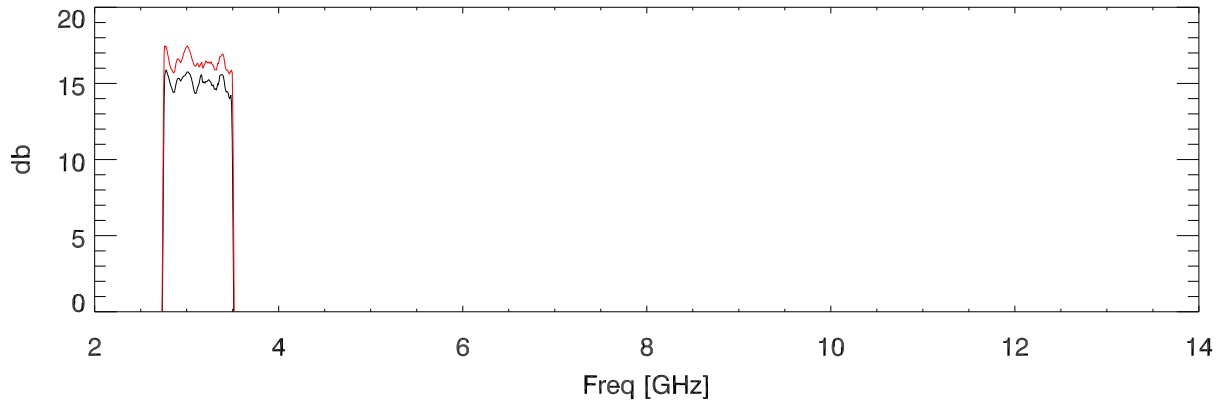
FilterBox Sparams. filtNum=3, cfr=3125 (2775-3475) bandpass. S21
