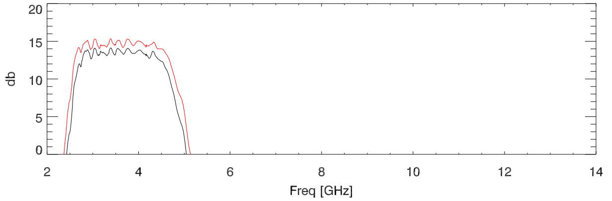
FilterBox Sparams. filtNum=2, cfr=3590 (2940-4240) bandpass. S21
