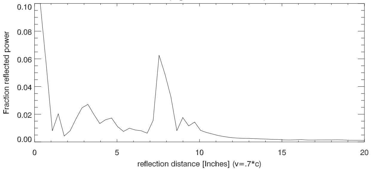
Acf S11 (lag distance in inches)
