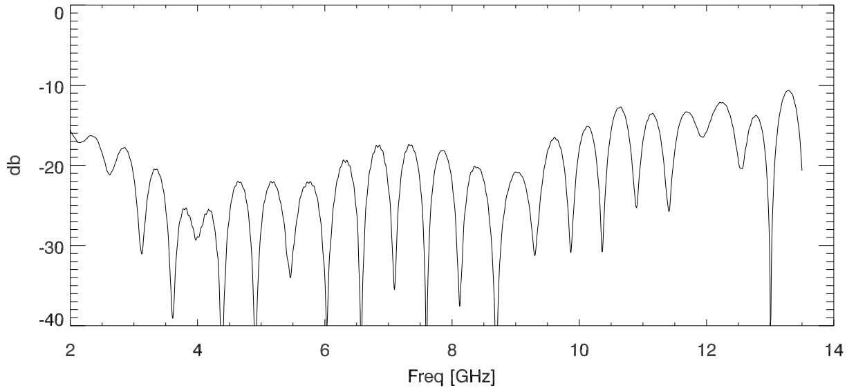
S11 polX straight thru filter
