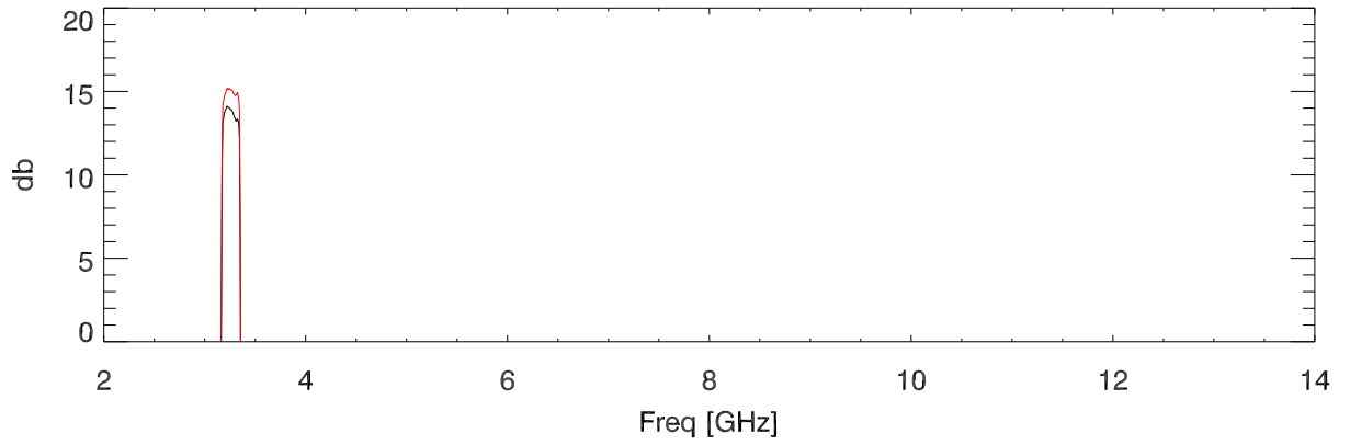
FilterBox Sparams. filtNum=4, cfr=3260 (3180-3340) bandpass. S21
