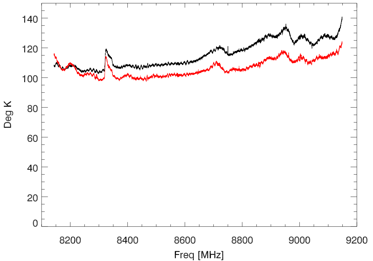
17jan22 Measured Tsys vs freq (using calOffs)
