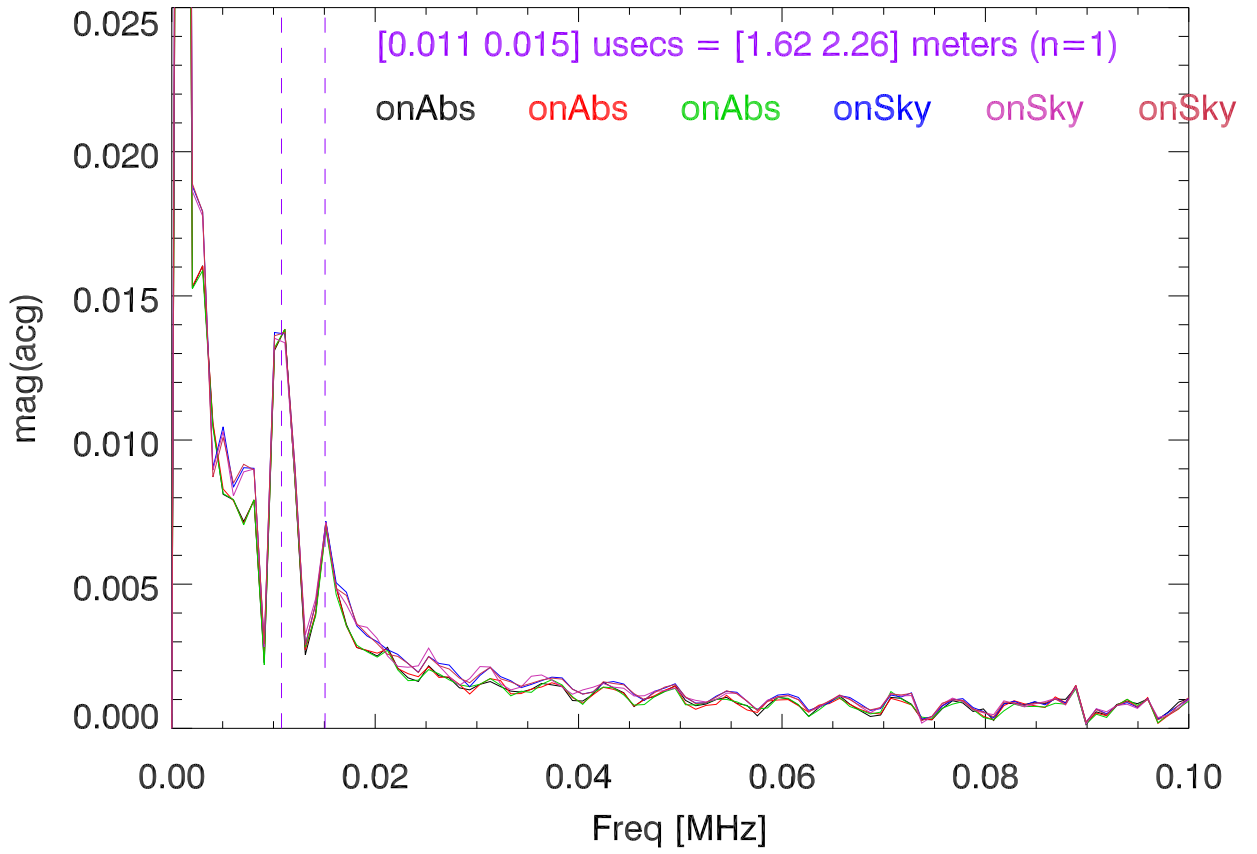
220624 acf of calRatio spectra showing ripple spacing. PoIA
