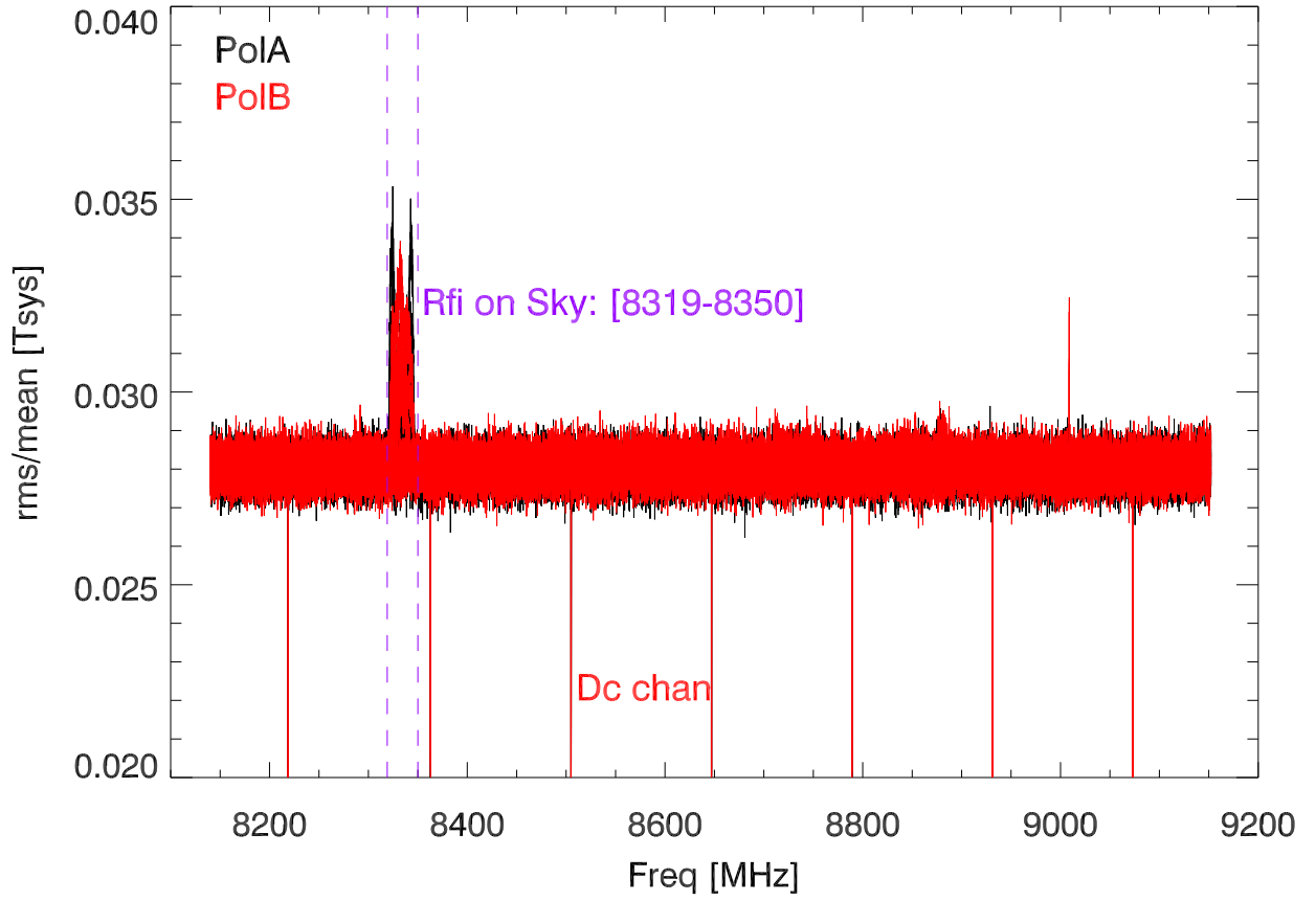
220624 Rms/mean by freqChan for calon,caloff spectra. OnSky
