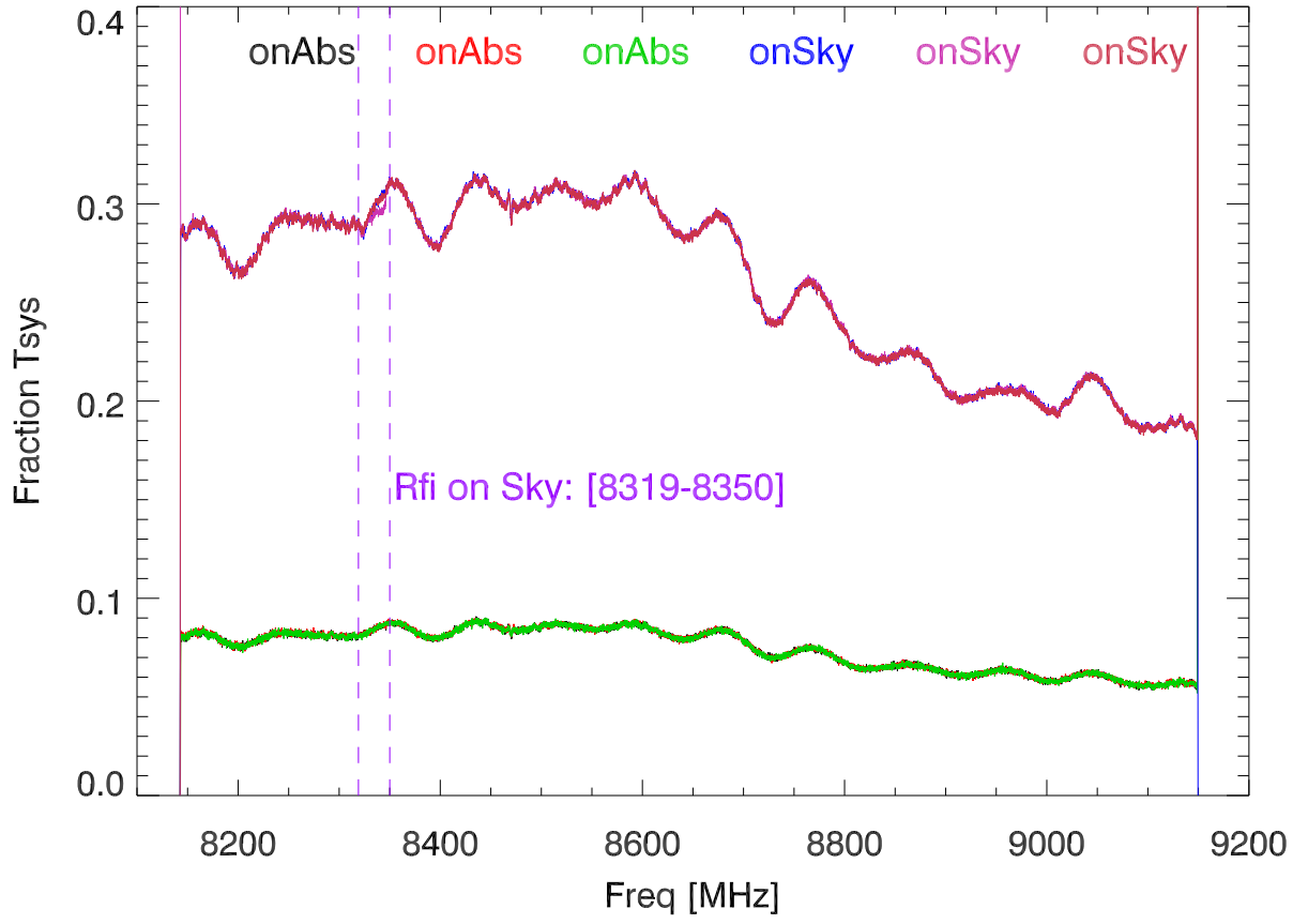
220624 CalDeflect/CalOff vs freq. PoIA
