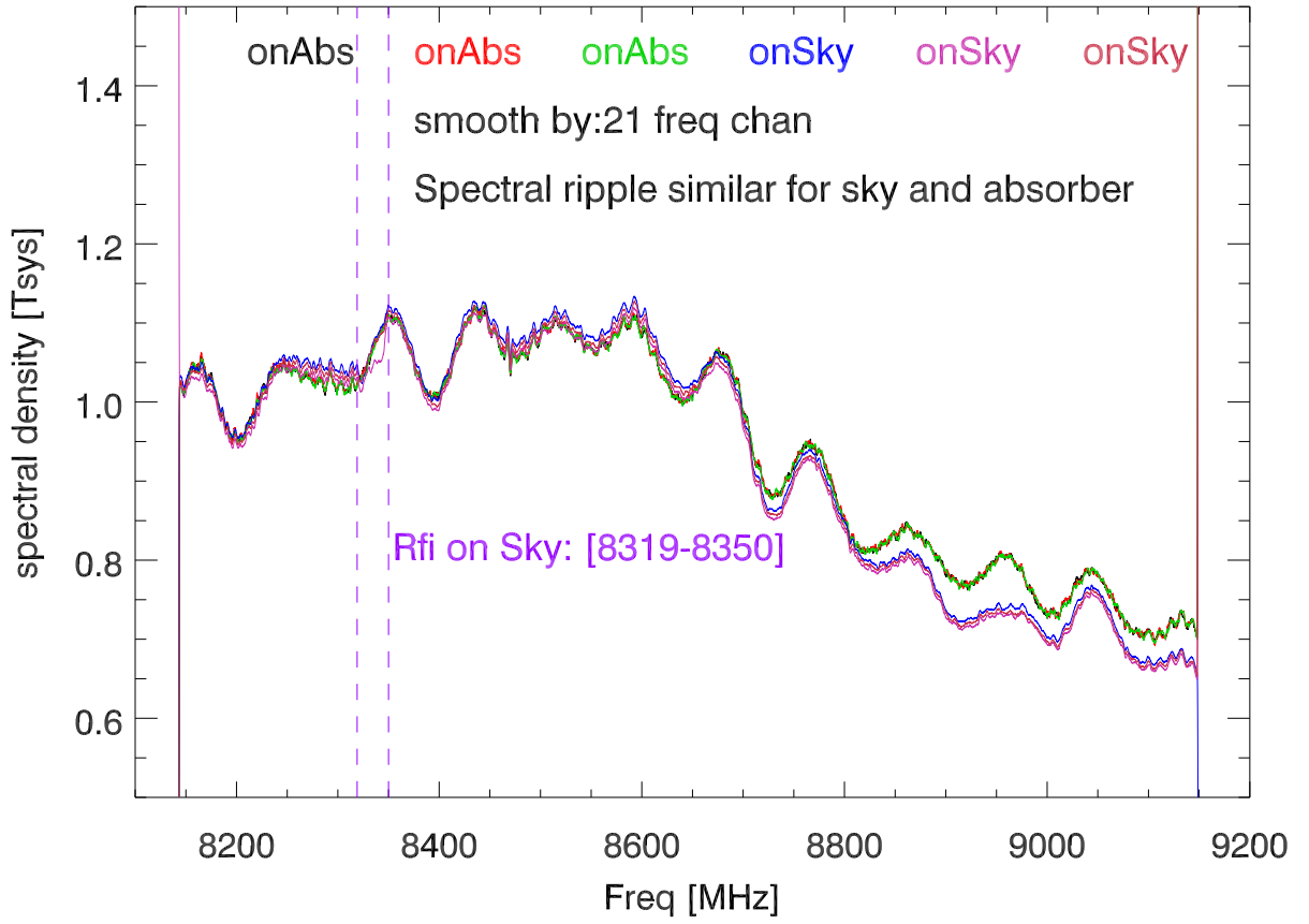
220624 Normalized CalDeflect/CalOff vs freq. PoIA
