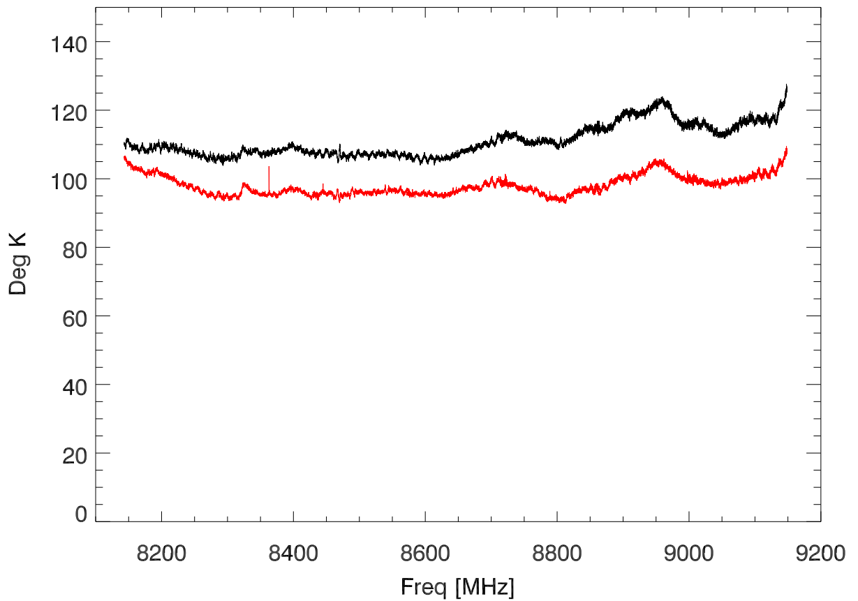
220624 Measured Tsys vs freq (using calOffs)
