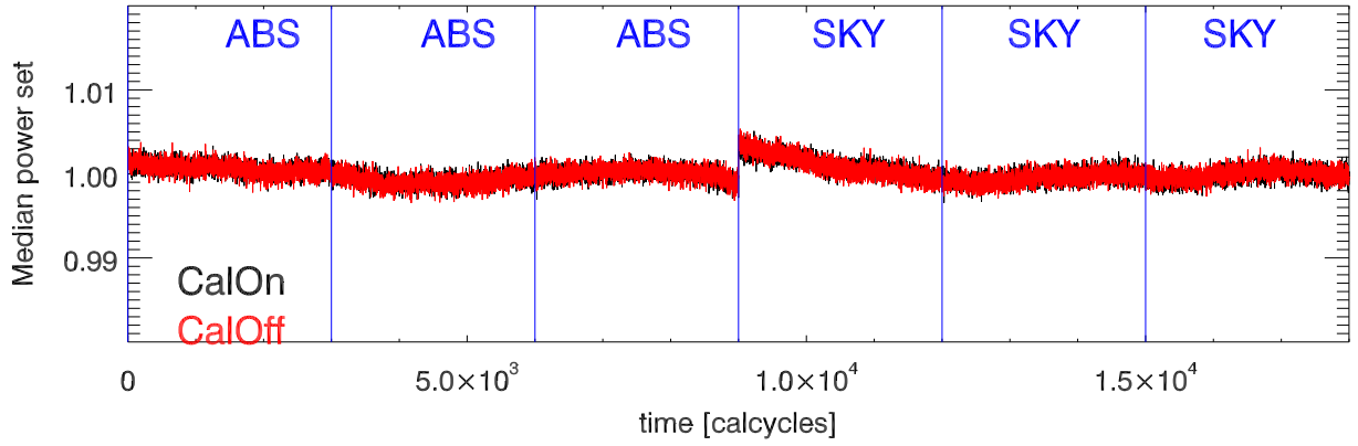
220624 measureCal totPwrVsTm. 8505 Mhz PoIA
