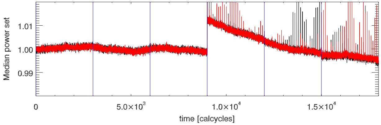
8789 Mhz PoIB
