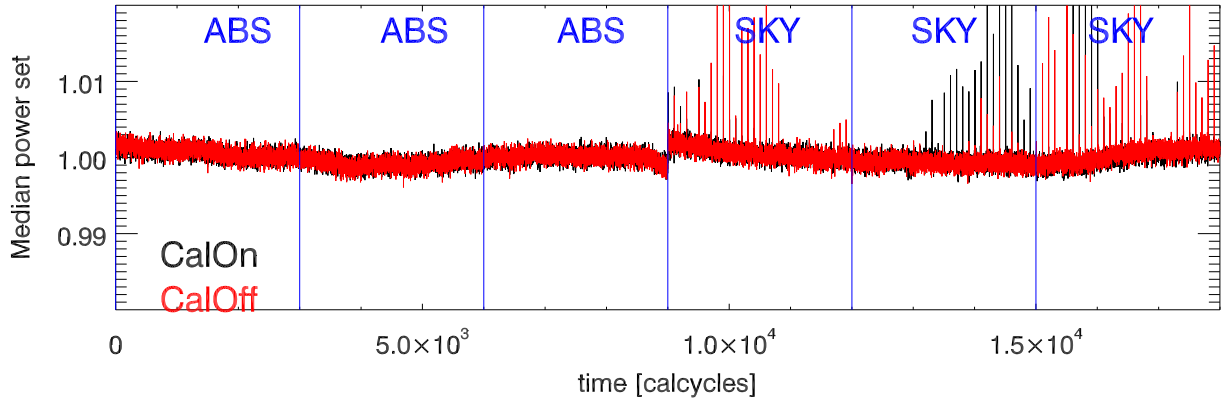
220624 measureCal totPwrVsTm. 8789 Mhz PoIA
