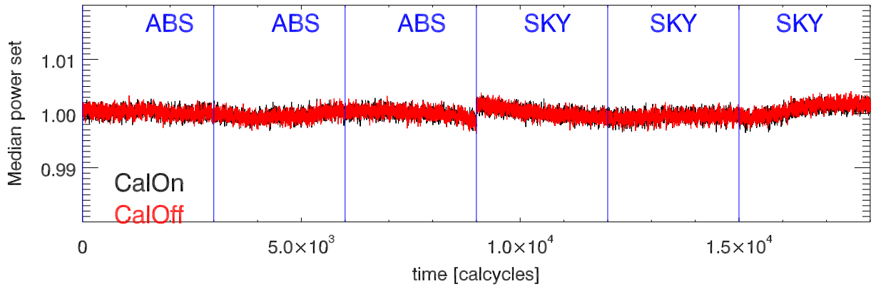
220624 measureCal totPwrVsTm. 9073 Mhz PolA
