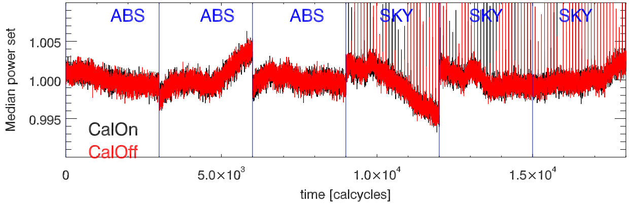
220607 measureCal totPwrVsTm. 8789 Mhz PoIA
