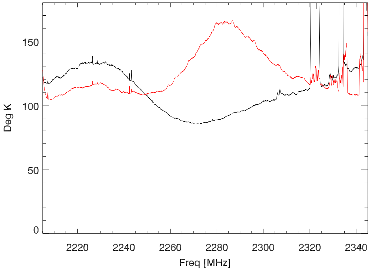
220607 Measured Sband Tsys vs freq (using calOffs)
