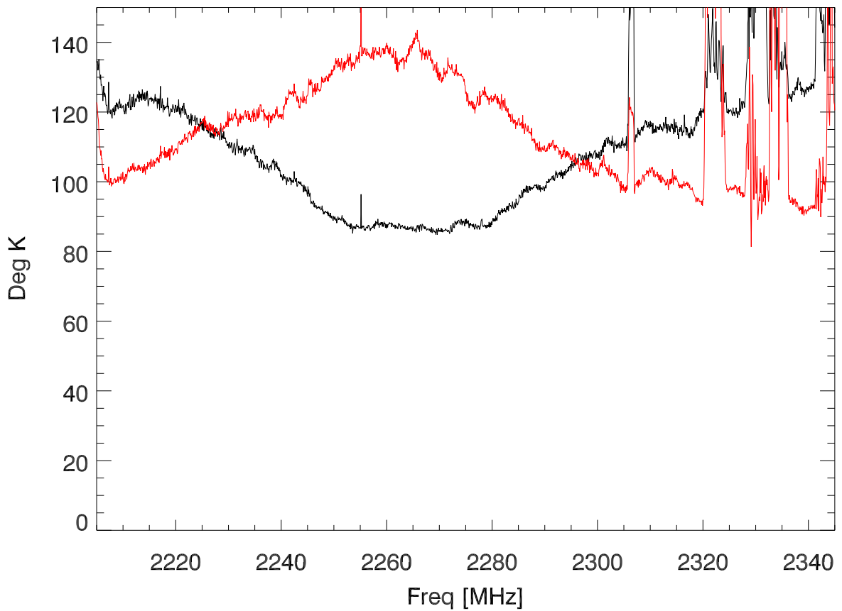
27may22 Measured Sband Tsys vs freq (using calOffs)
