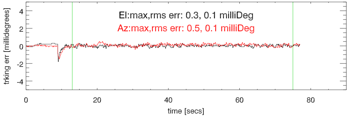
tracking error. Elvel and AzVel=.01 deg/sec
