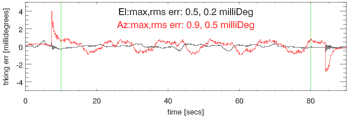
tracking error. Azvel=.1 deg/sec
