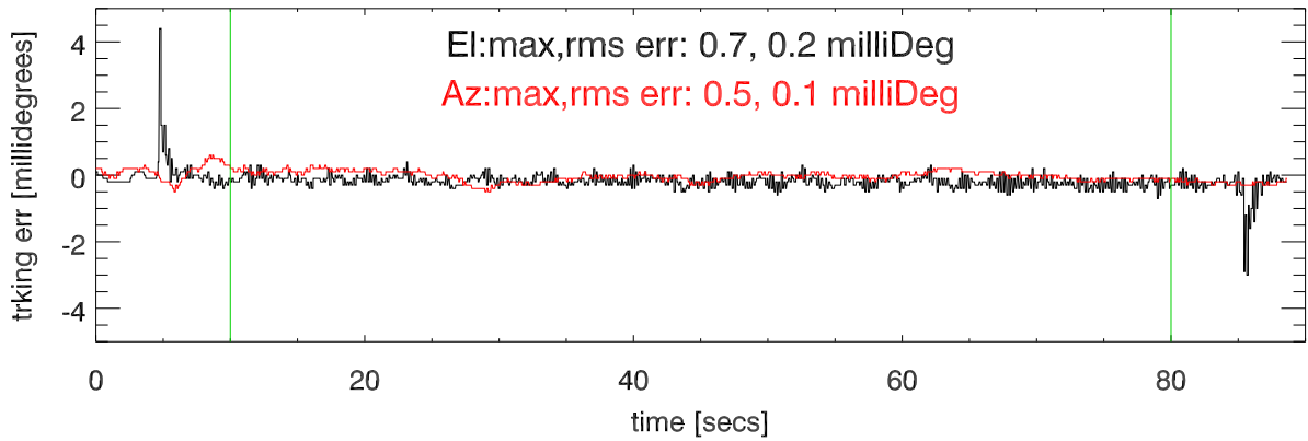
tracking error. Elvel=.1 deg/sec
