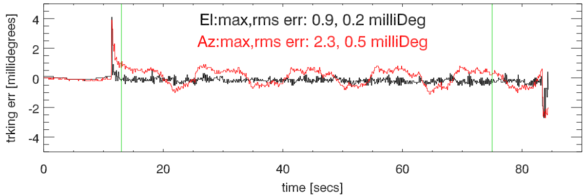
tracking error. Elvel anz AzVel=.1 deg/sec
