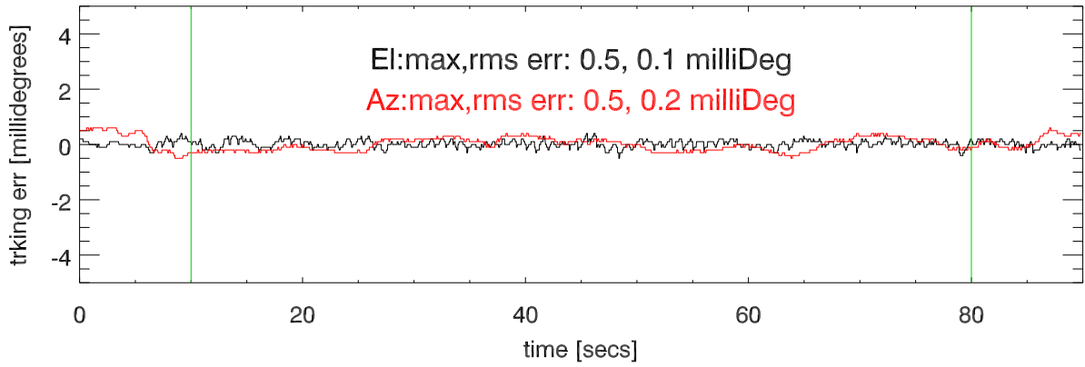
24jan11:VelResponse tracking error. Elvel=.001 deg/sec. (El=45 deg)
