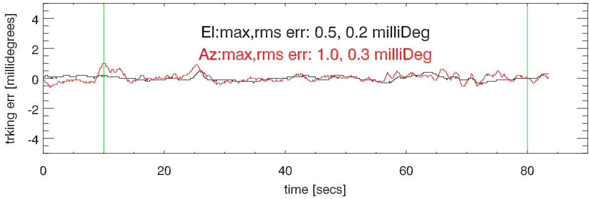
24jan11:VelResponse tracking error. Azvel=.001 deg/sec. (El=45 deg)
