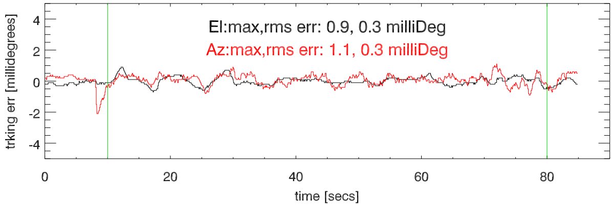
tracking error. Azvel=.01 deg/sec
