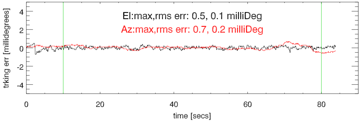
tracking error. Elvel=.01 deg/sec
