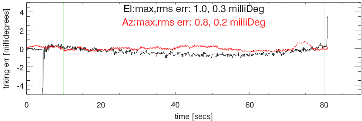
tracking error. Elvel=.4 deg/sec
