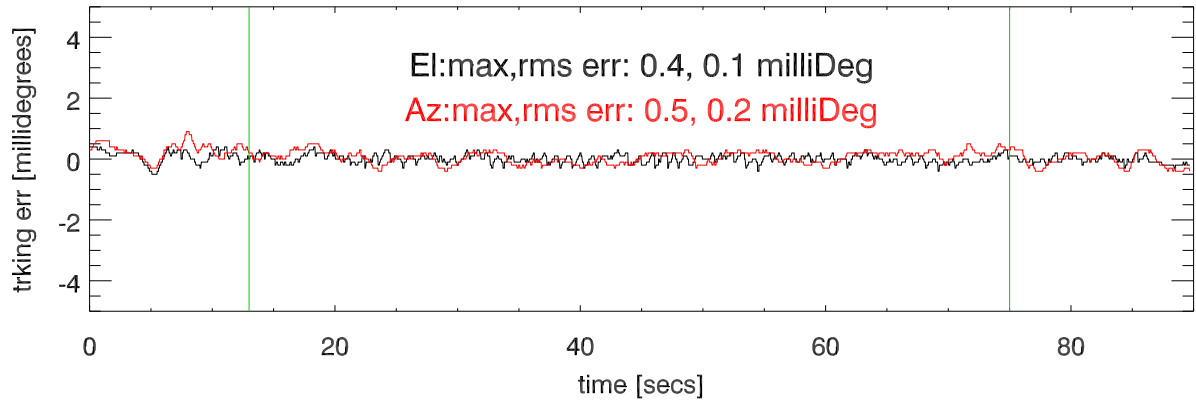
24jan11:VelResponse tracking error. Elvel and AzVel=.001 deg/sec. (El=45 deg)
