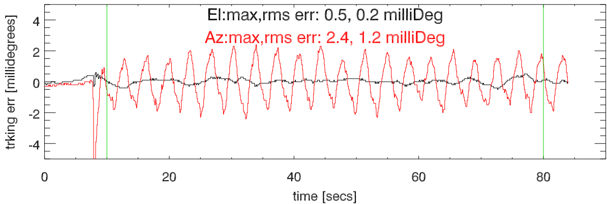
tracking error. Azvel=.4 deg/sec
