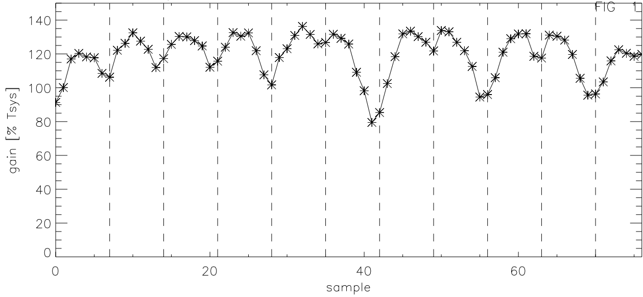
10may06 sbnTx J2253+161focus curve vs sample polB
