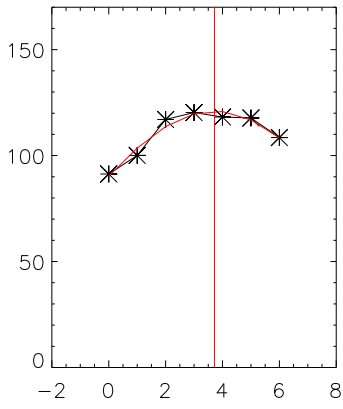
polBGauss fits to gain versus minute of each star FIG 2
