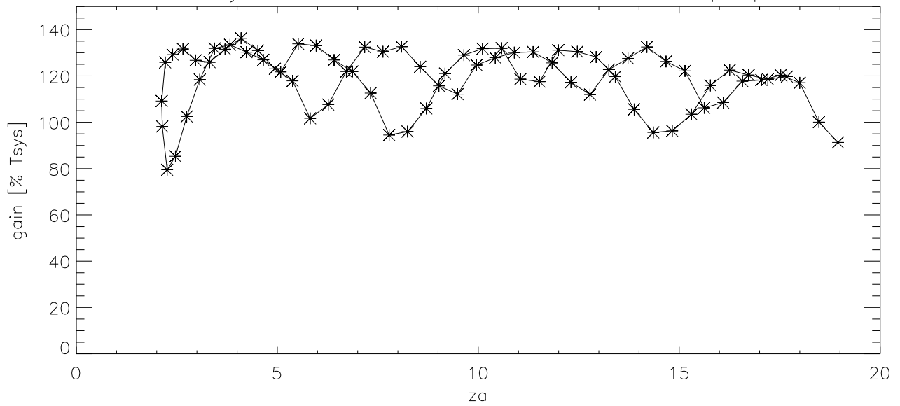
10may06 sbnTx J2253+161focus curve vs sample polB
