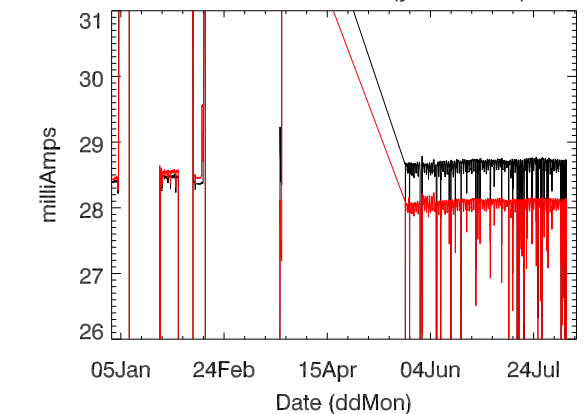
12m Drain current (year 2023)
