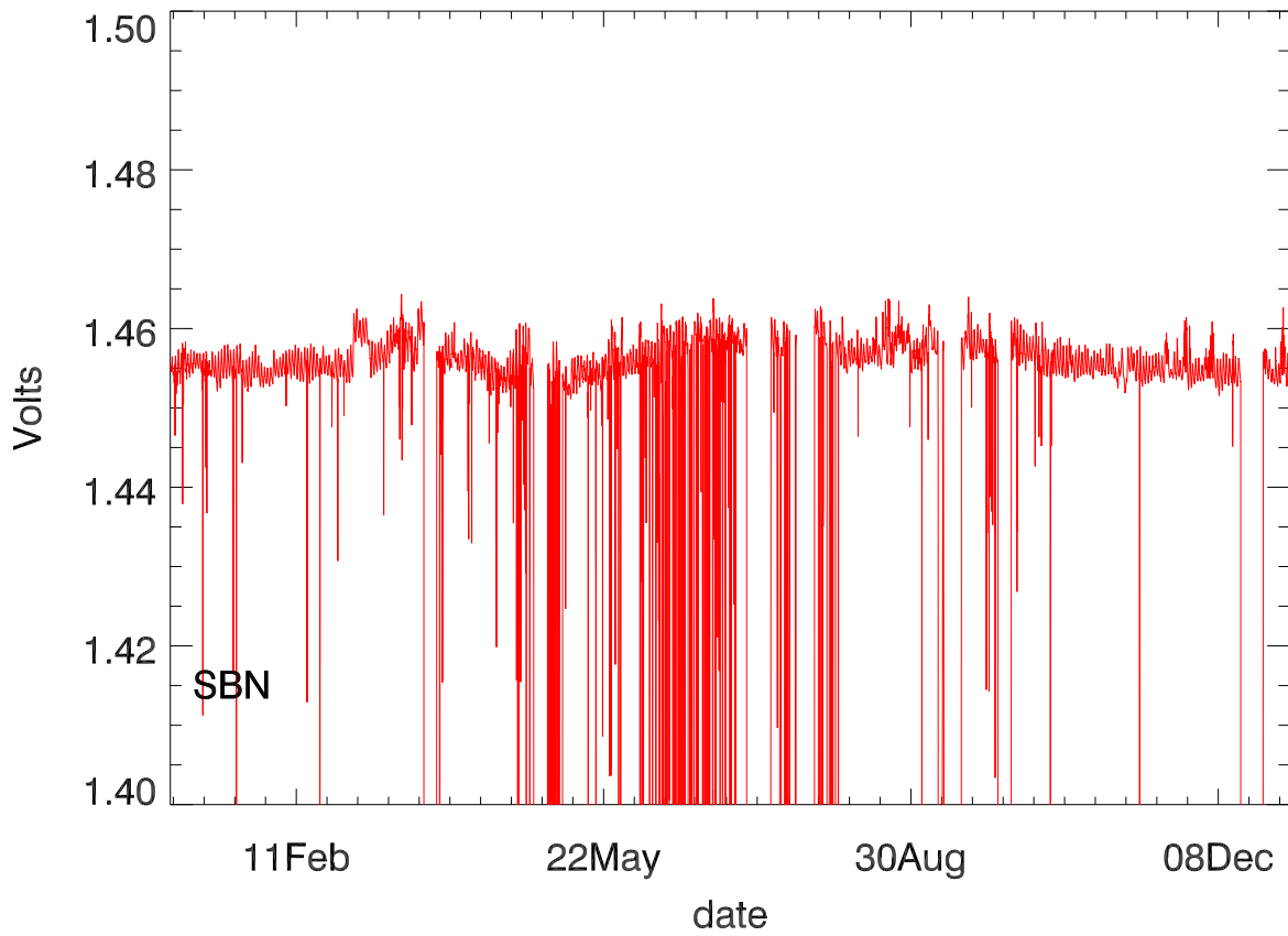
Dewar voltage stage 2 (year 2014)
