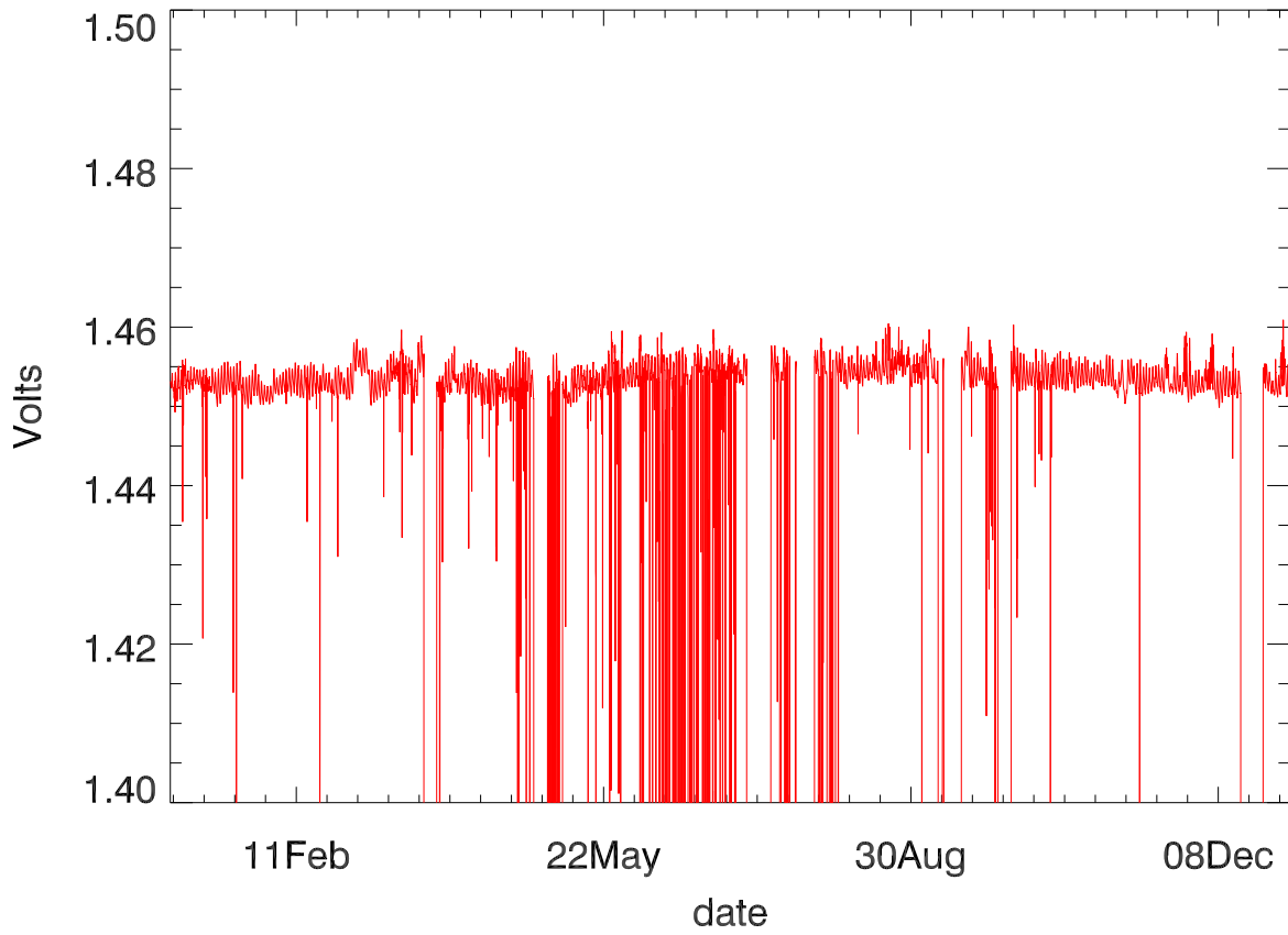
Dewar voltage stage 1 (year 2014)
