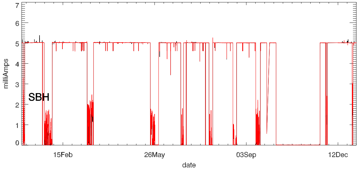
Dewar Current stage 3 (year 2017)
