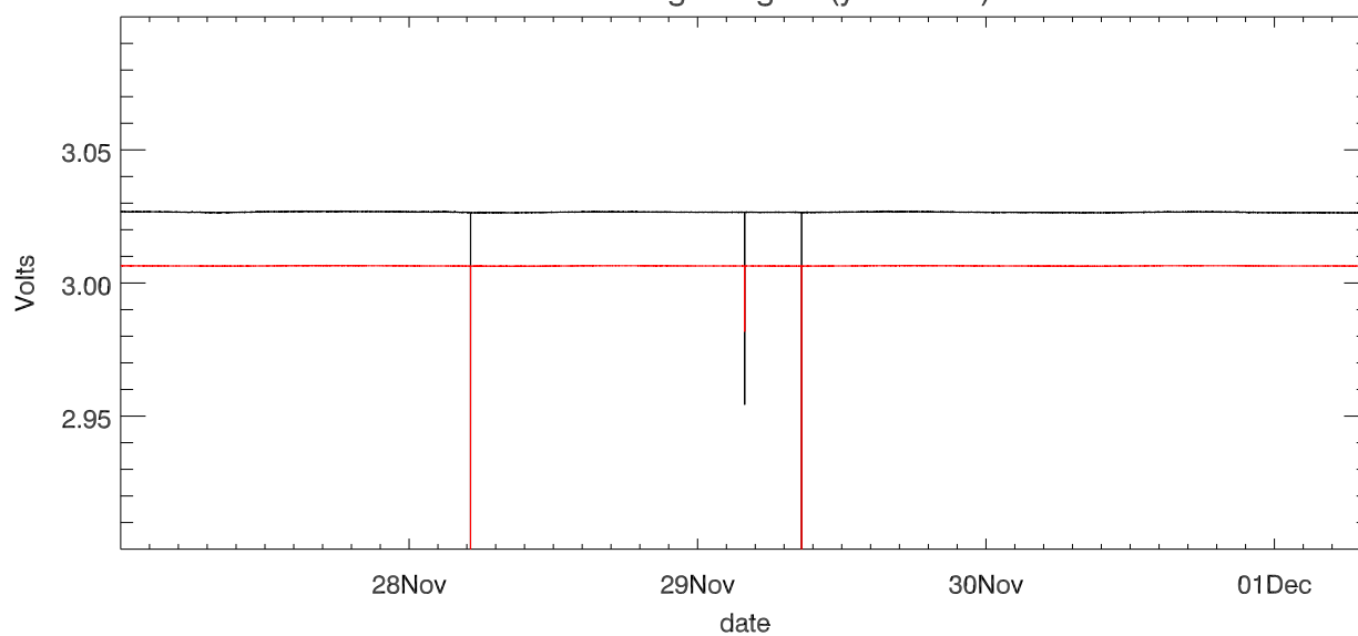
Dewar voltage stage 2 (year 2020)
