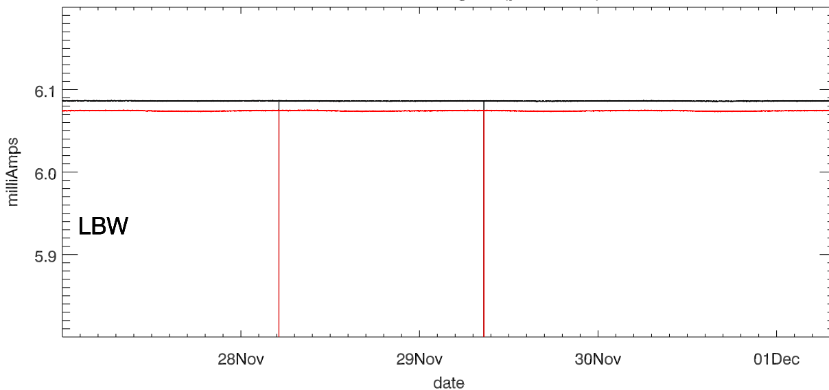
Dewar Current stage 3 (year 2020)
