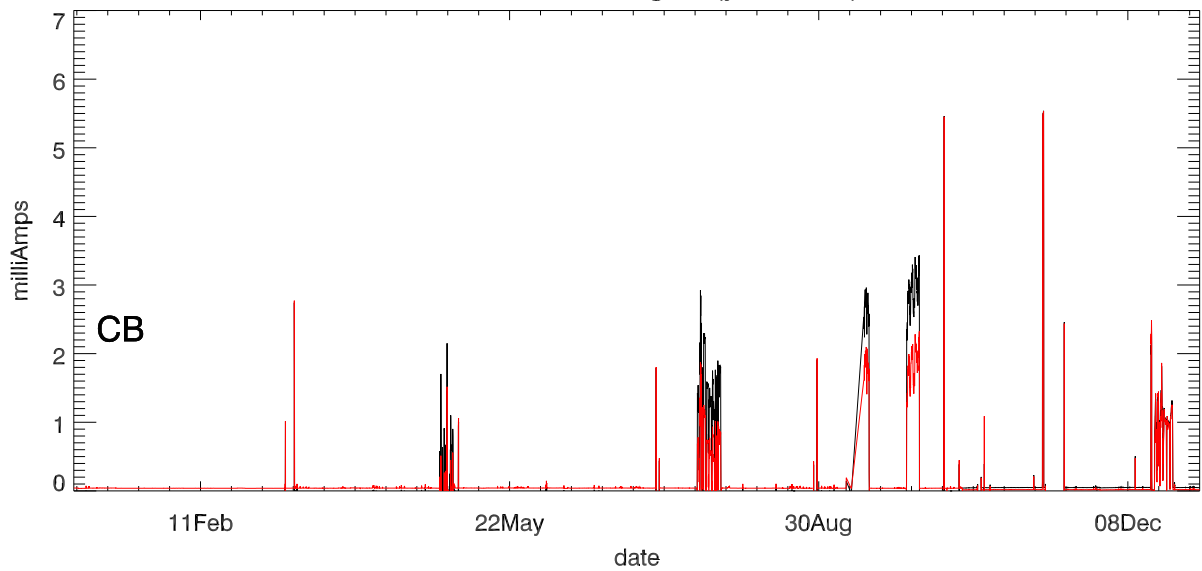
Dewar Current stage 3 (year 2014)
