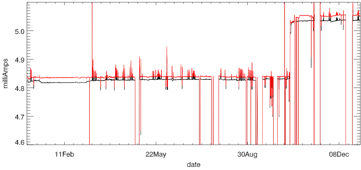
Dewar Current stage 1 (year 2014)
