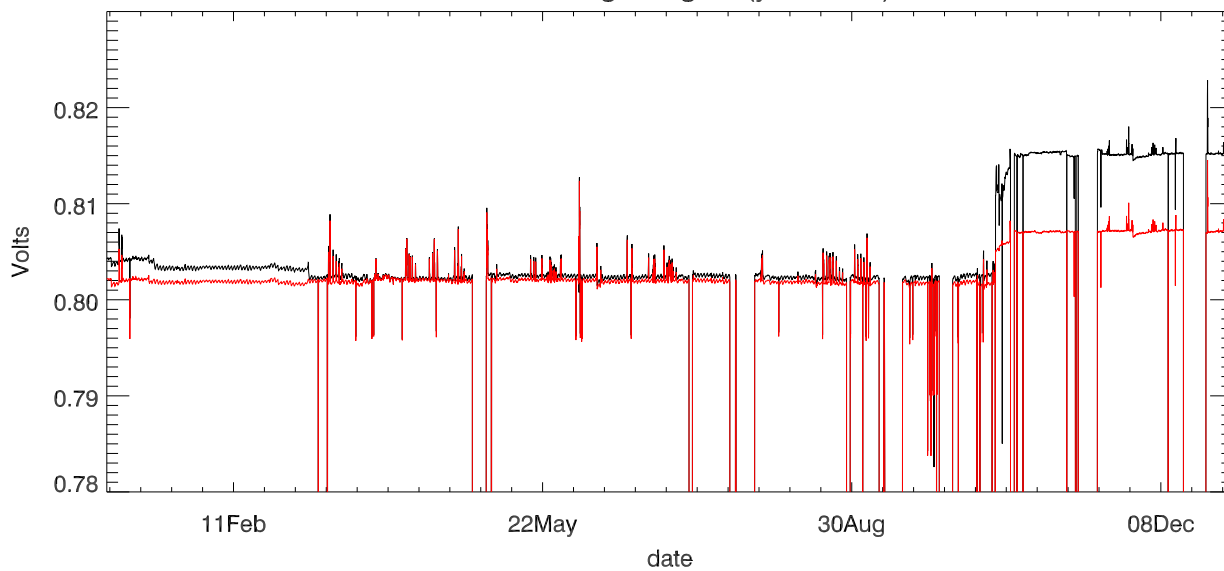
Dewar voltage stage 1 (year 2014)
