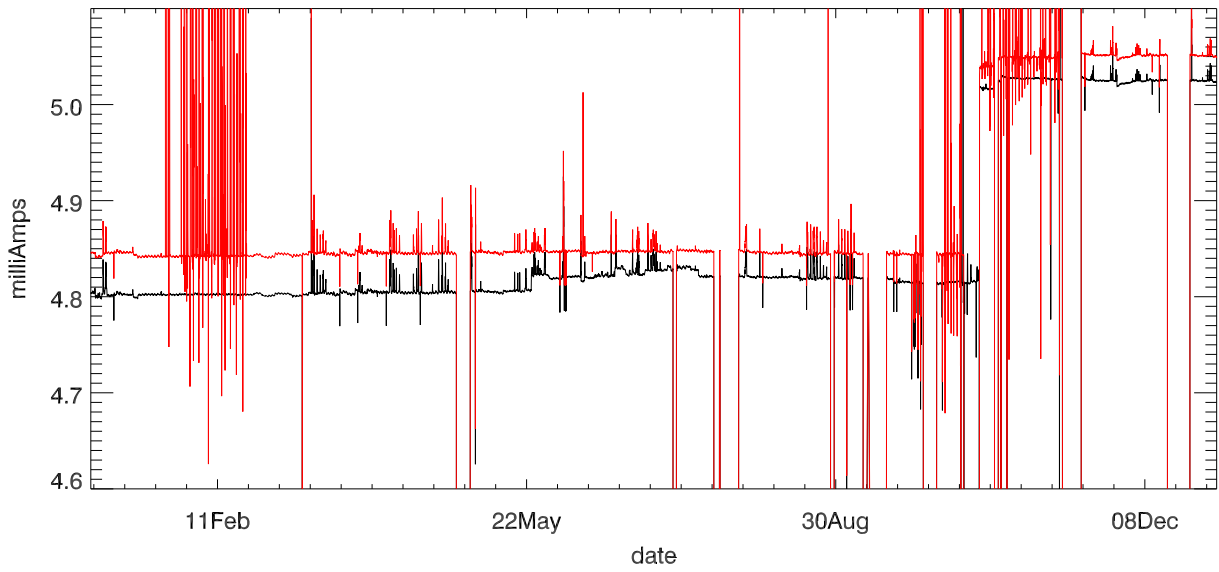
Dewar Current stage 2 (year 2014)
