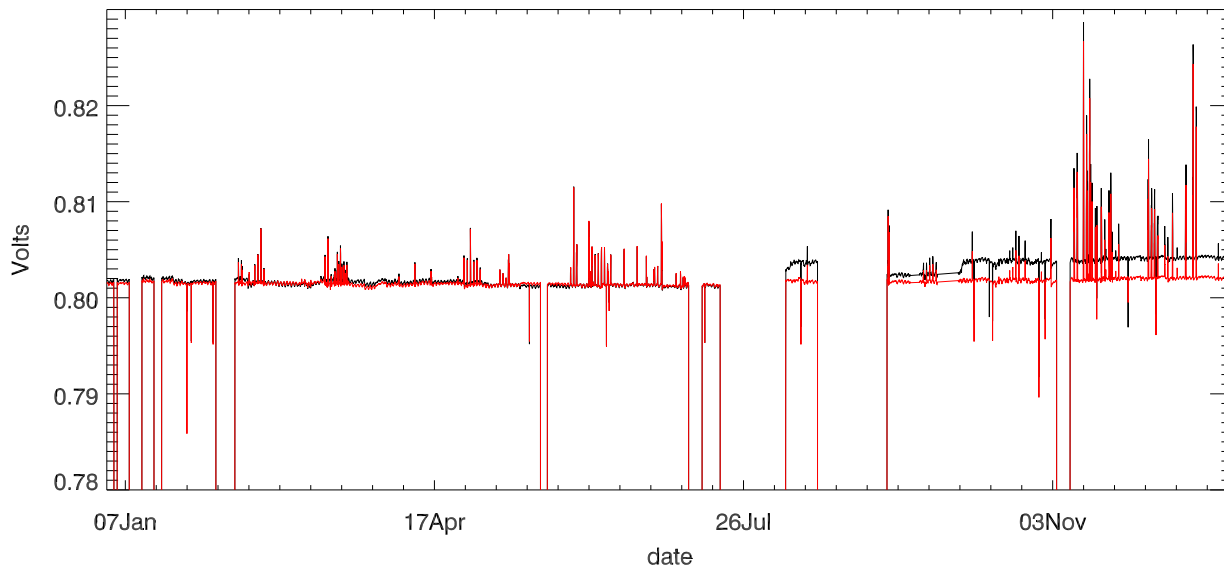
Dewar voltage stage 1 (year 2013)
