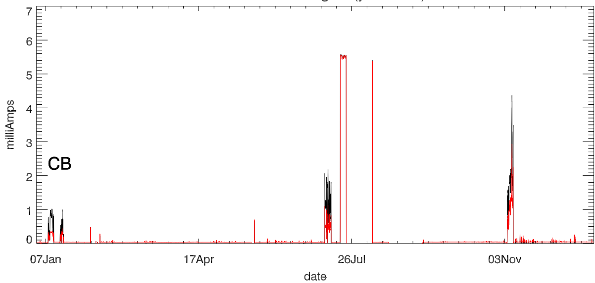
Dewar Current stage 3 (year 2013)
