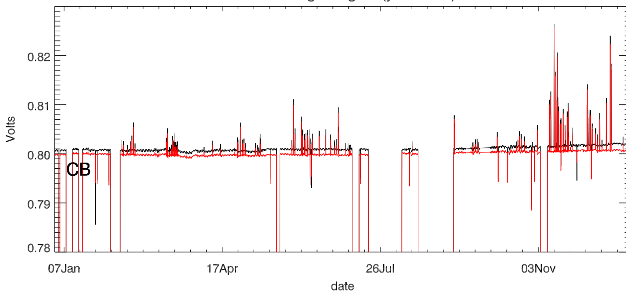
Dewar voltage stage 3 (year 2013)
