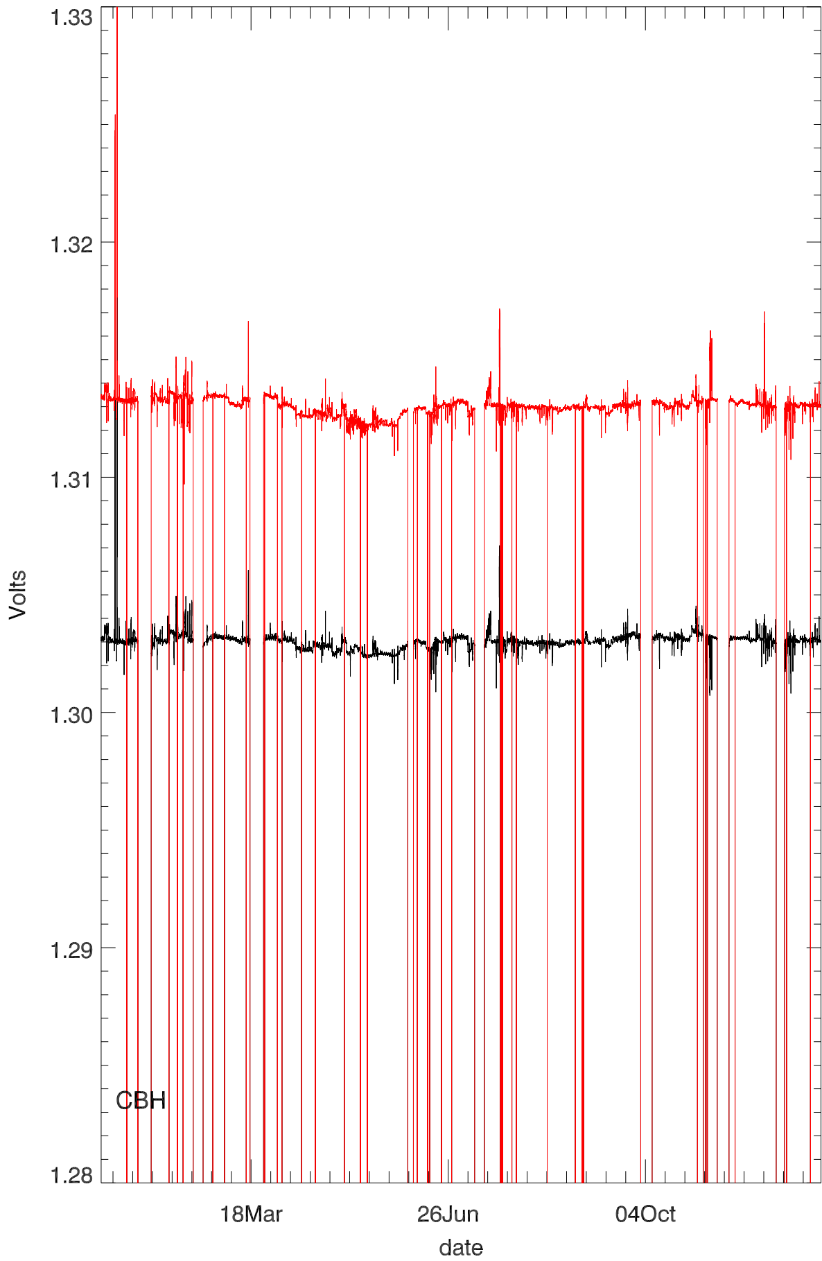
Dewar voltage stage 1 (year 2015)
