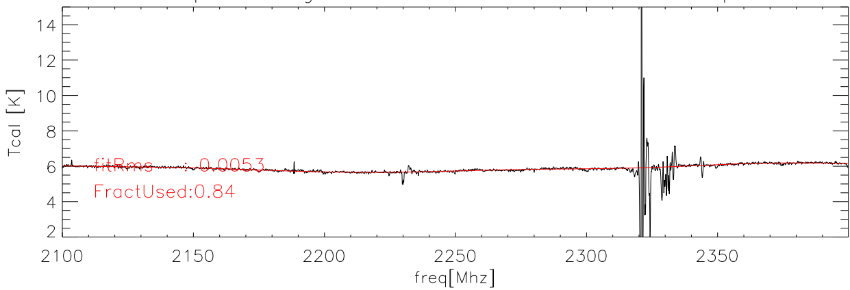
26sep08 Averaged data and fit for Tcal Kelvins hxcal polA
