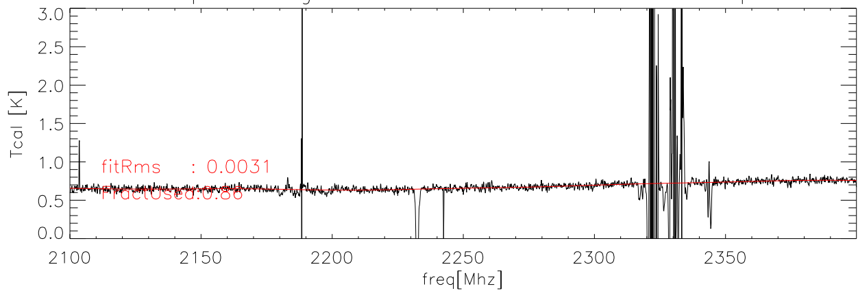
26sep08 Averaged data and fit for Tcal Kelvins I90cal polB
