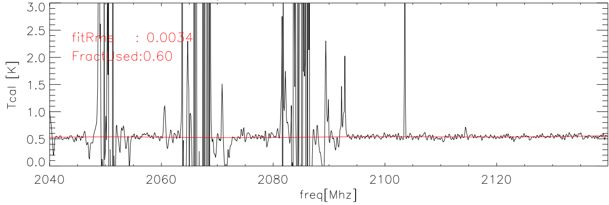
26sep08 Averaged data and fit for Tcal Kelvins I90cal polB
