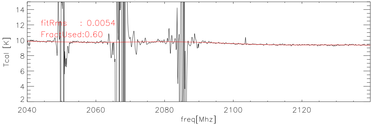
26sep08 Averaged data and fit for Tcal Kelvins hcal polB
