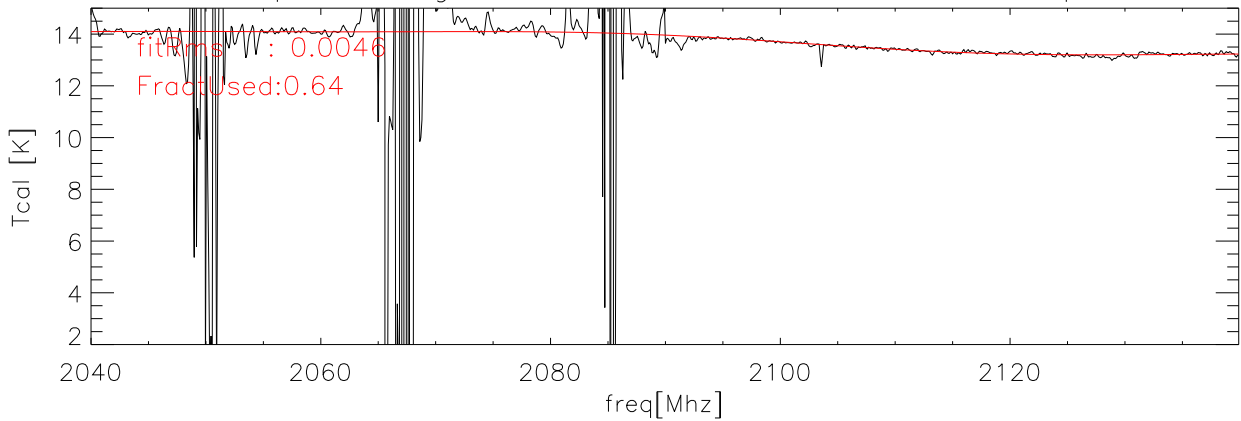
26sep08 Averaged data and fit for Tcal Kelvins hxcal polB
