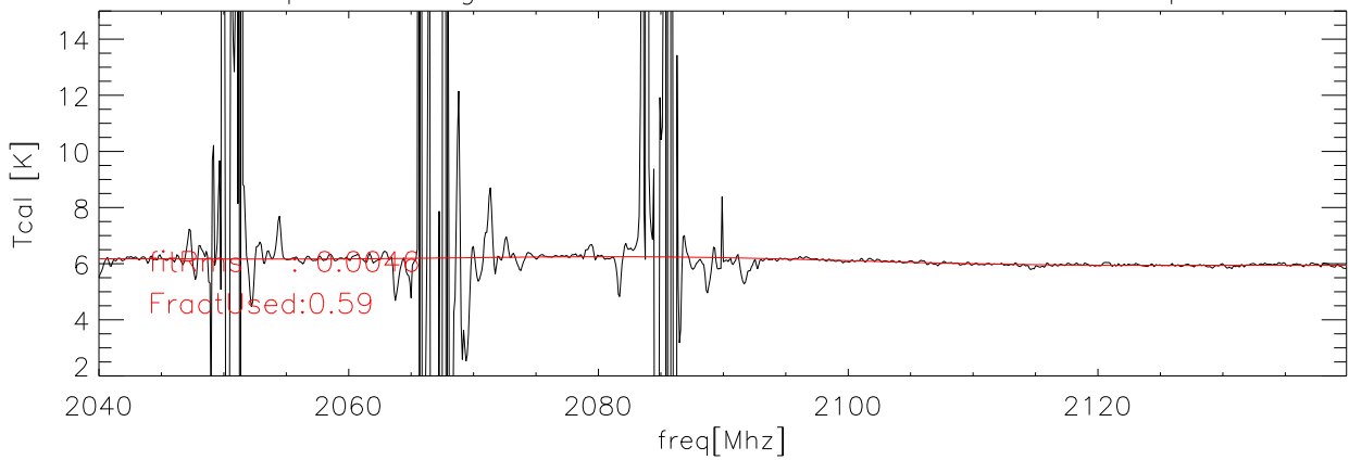
26sep08 Averaged data and fit for Tcal Kelvins lcor polA
