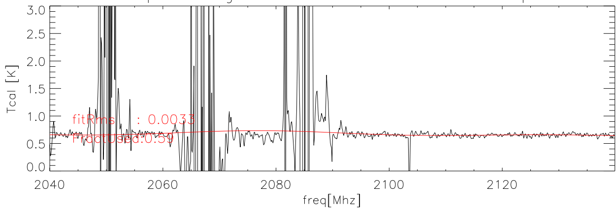
26sep08 Averaged data and fit for Tcal Kelvins lxcal polA
