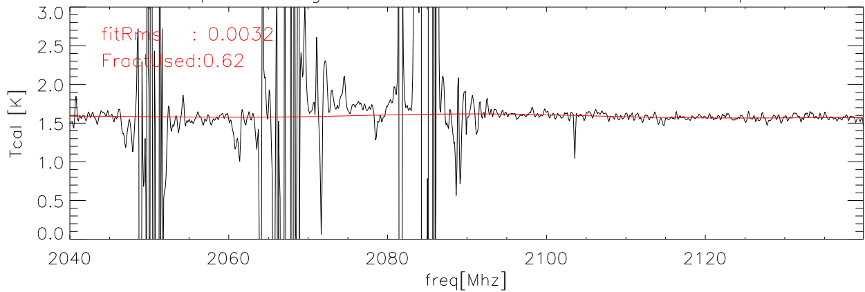
26sep08 Averaged data and fit for Tcal Kelvins lxcal polB
