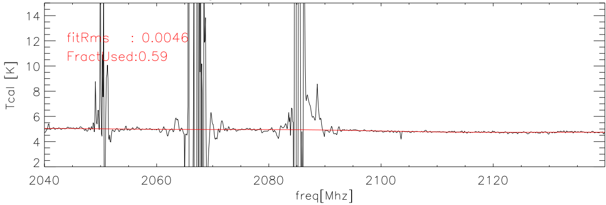
26sep08 Averaged data and fit for Tcal Kelvins h90cal polB
