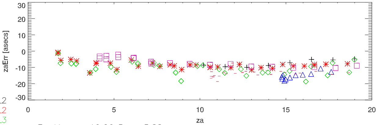
Point error new rcvr (out and in focus) za error vs za
