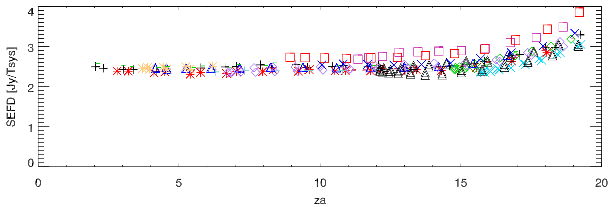
Sefd
