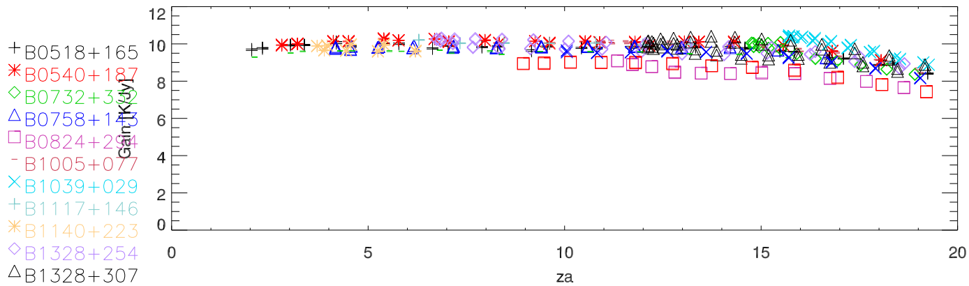
Gain K/Jy
